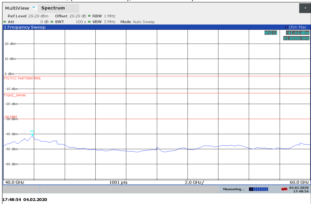
Plot 26: 40 GHz – 60 GHz, (valid for all modes), vertical / horizontal polarization
