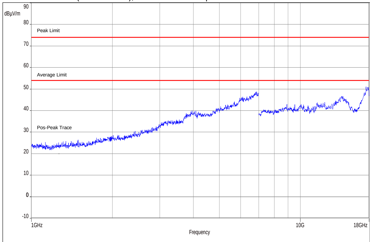
Plot 21: 1 GHz – 18 GHz (Mode DMP06), vertical / horizontal polarization
