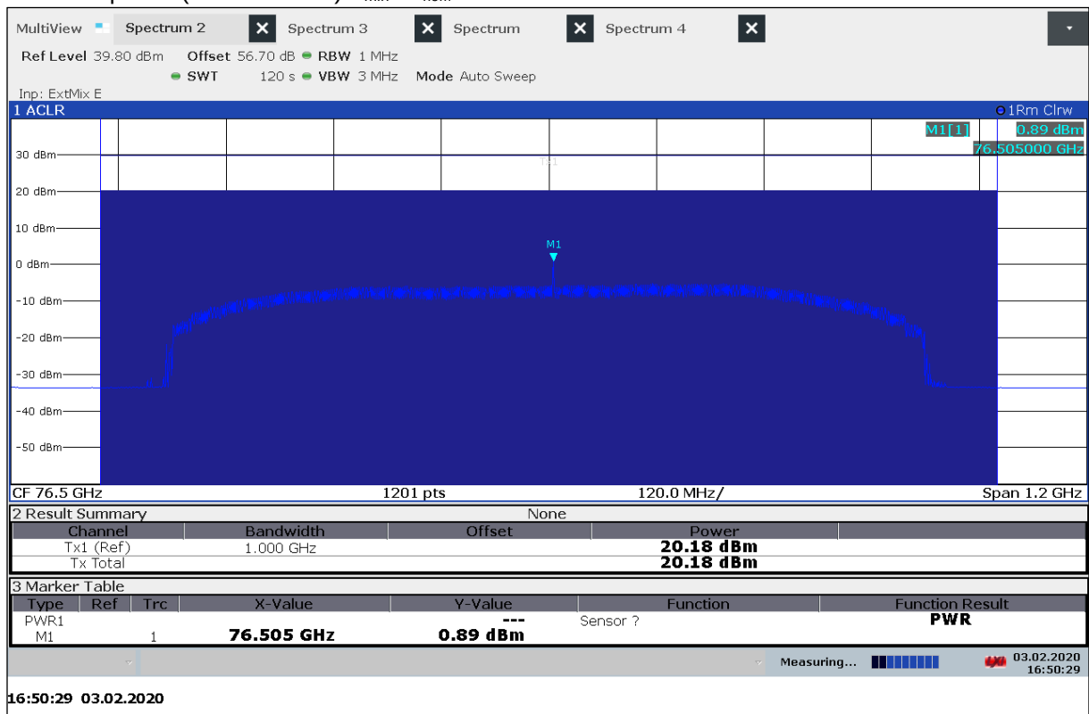
Plot 10: Mean power (Mode DMP07) T_{\min} / V_{\text{nom}}
