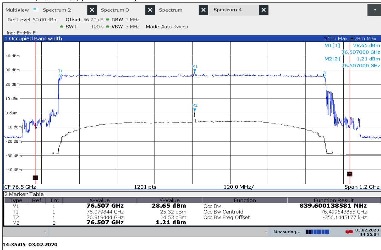
Plot 33: OBW, T_{\min} / V_{\text{nom}} , (Mode DMP07)
