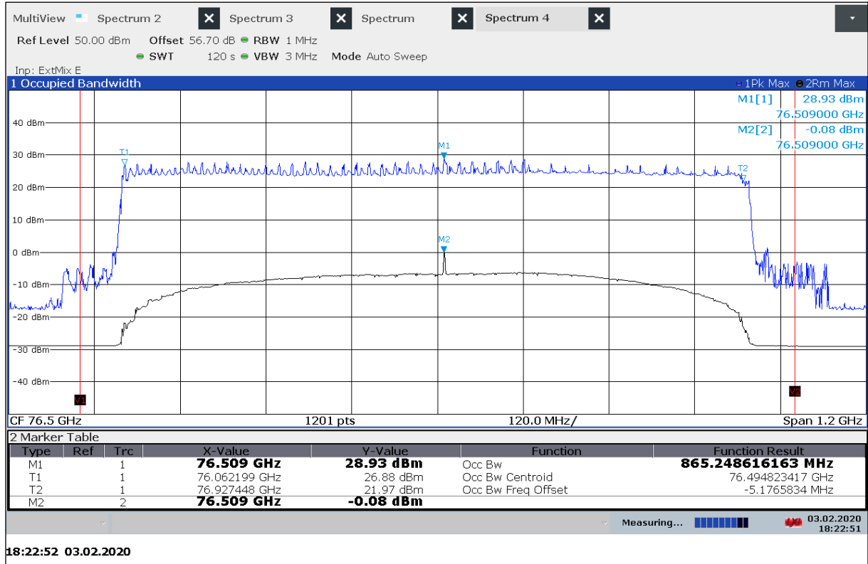
Plot 52: OBW, T_{\max} / V_{\text{nom}} , (Mode DMP06)
