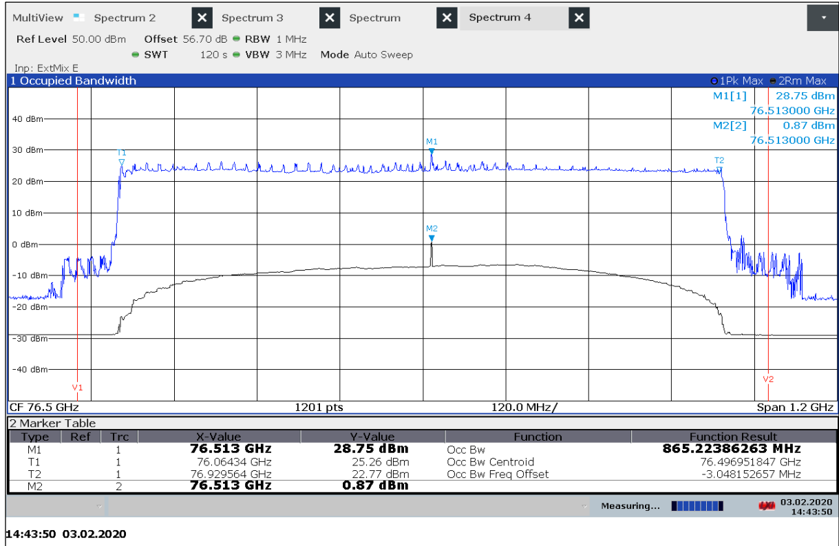
Plot 3: OBW, Radiated peak power, PSD (Mode DMP06) T_{min} / V_{nom}
