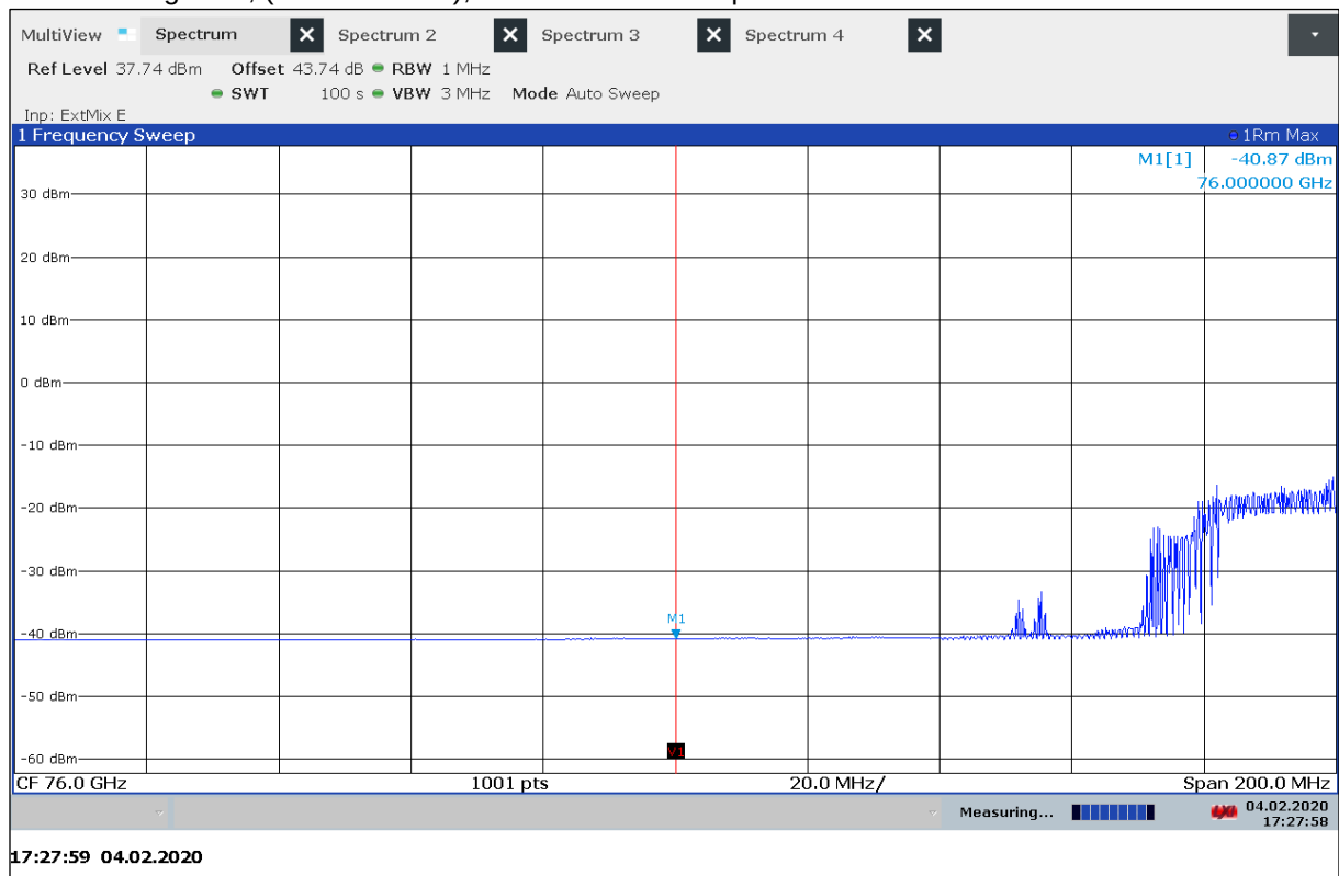
Plot 14: Band edge low, (Mode DMP07), vertical / horizontal polarization
