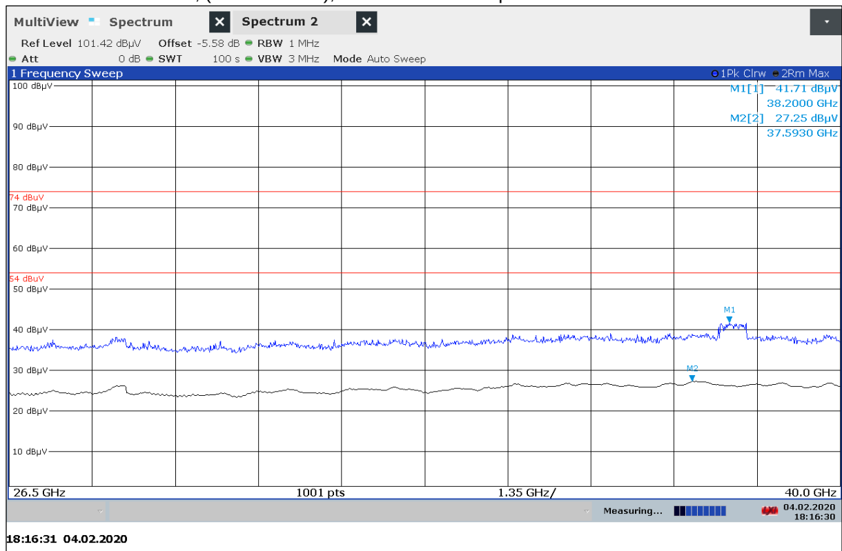
Plot 24: 26.5 GHz – 40 GHz, (Mode DMP06), vertical / horizontal polarization
