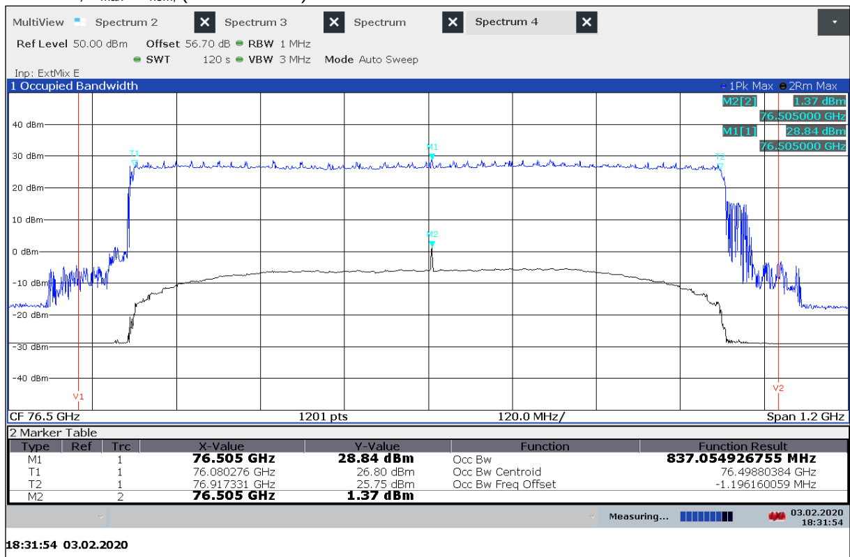
Plot 53: OBW, T_{\max} / V_{\text{nom}} , (Mode DMP07)
