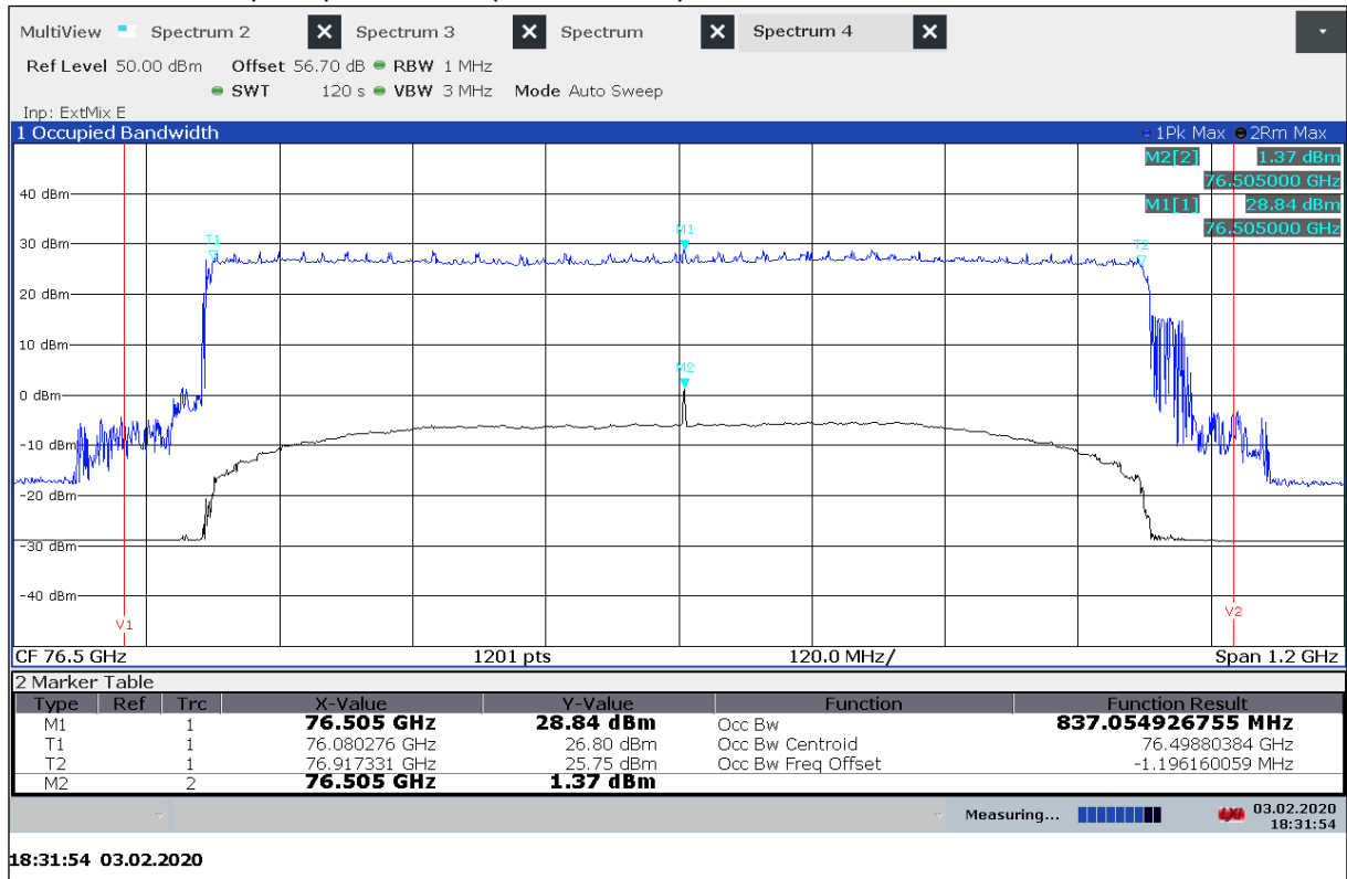
Plot 6: OBW, Radiated peak power, PSD (Mode DMP07) T_{\max} / V_{\text{nom}}
