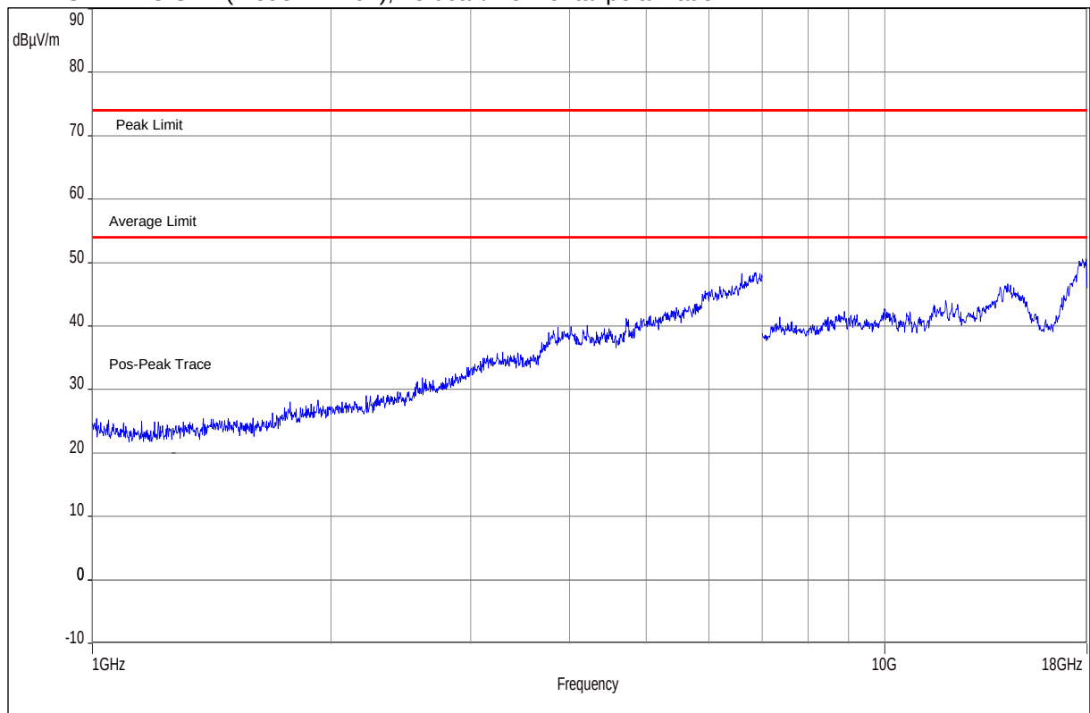
Plot 22: 1 GHz – 18 GHz (Mode DMP07), vertical / horizontal polarization
