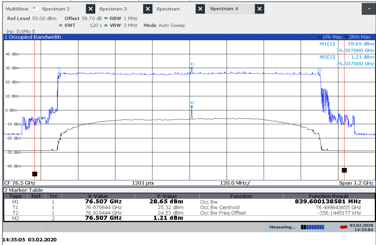
Plot 4: OBW, Radiated peak power, PSD (Mode DMP07) T_{min} / V_{nom}
