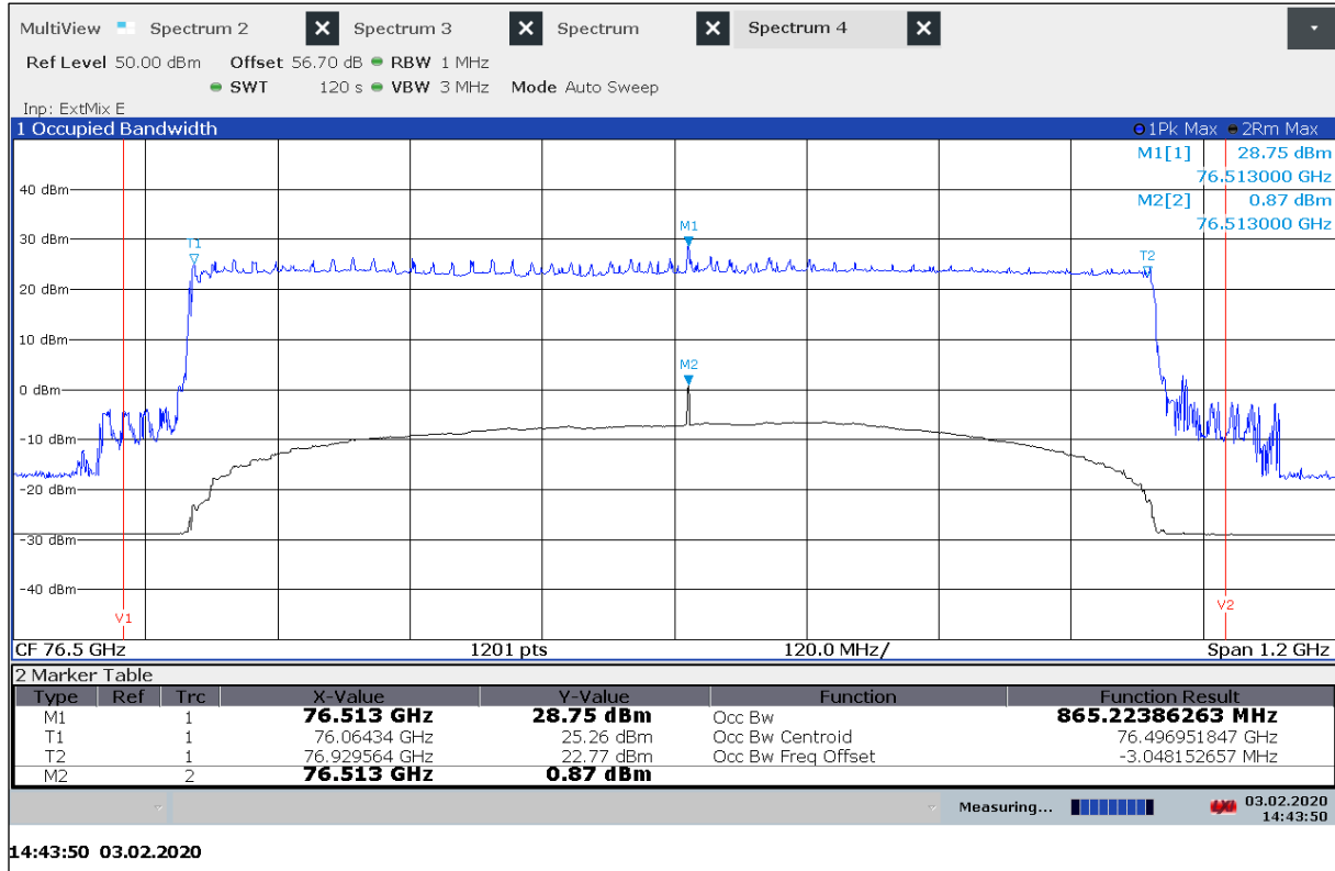
Plot 32: OBW, T_{\min} / V_{\text{nom}} , (Mode DMP06)
