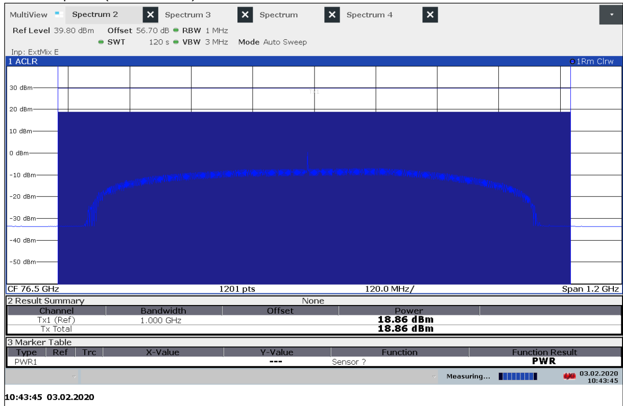
Plot 11: Mean power (Mode DMP06) T_{\max} / V_{\text{nom}}
