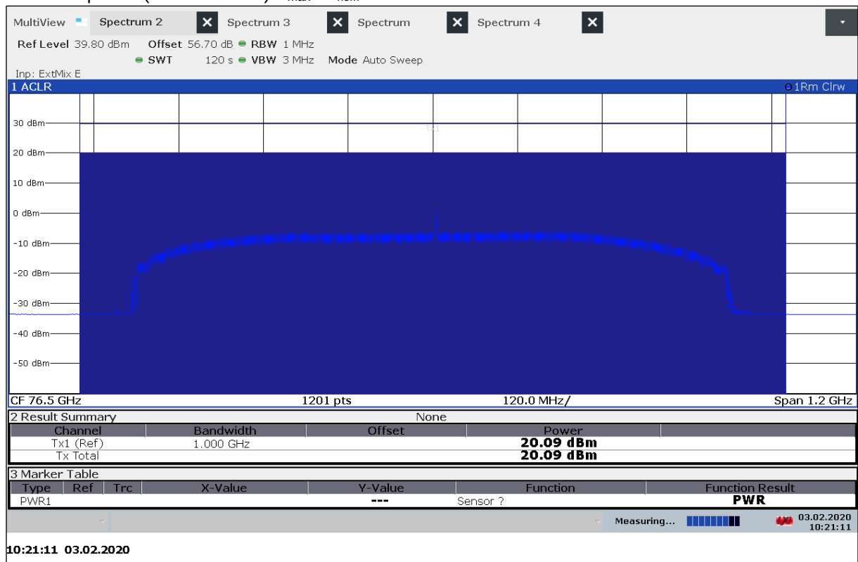
Plot 12: Mean power (Mode DMP07) T_{\max} / V_{\text{nom}}
