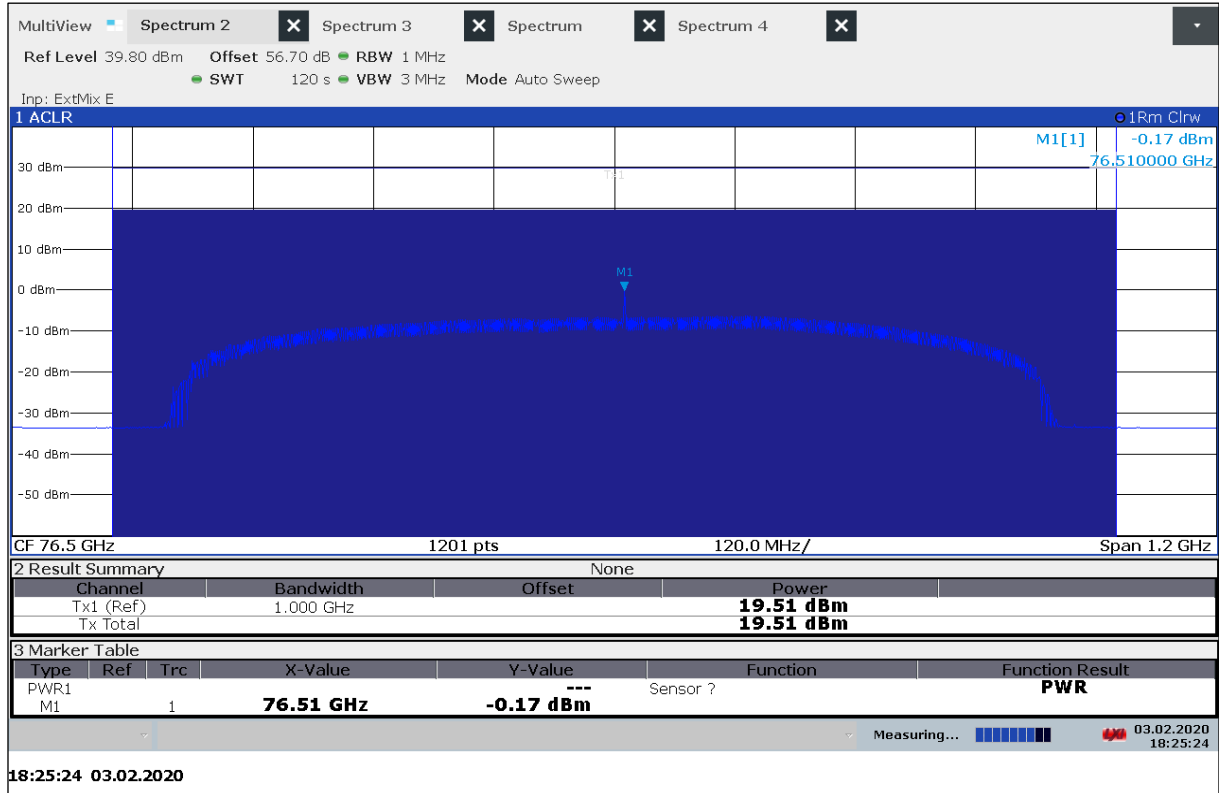
Plot 9: Mean power (Mode DMP06) T_{\min} / V_{\text{nom}}
