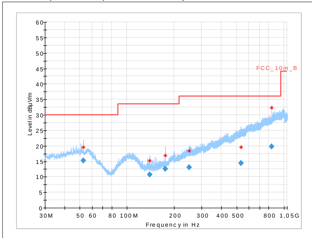
Plot 19: 30 MHz – 1 GHz, (Mode DMP06), vertical / horizontal polarization
