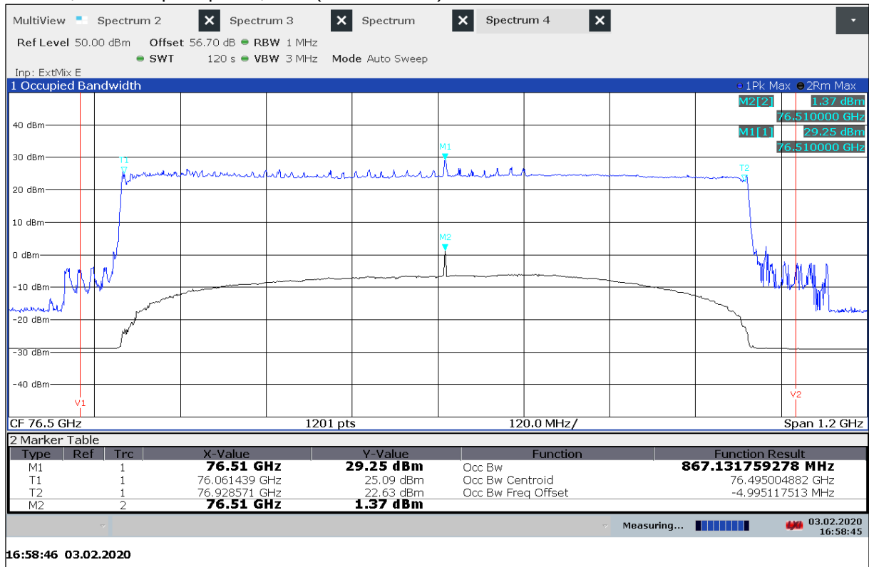
Plot 1: OBW, Radiated peak power, PSD (Mode DMP06) T_{nom} / V_{min-max}
