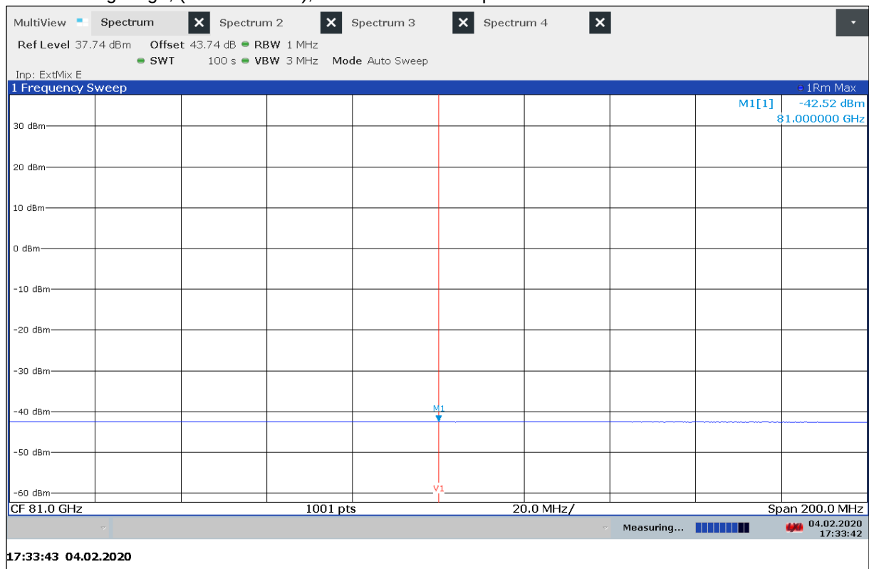
Plot 16: Band edge high, (Mode DMP07), vertical / horizontal polarization
