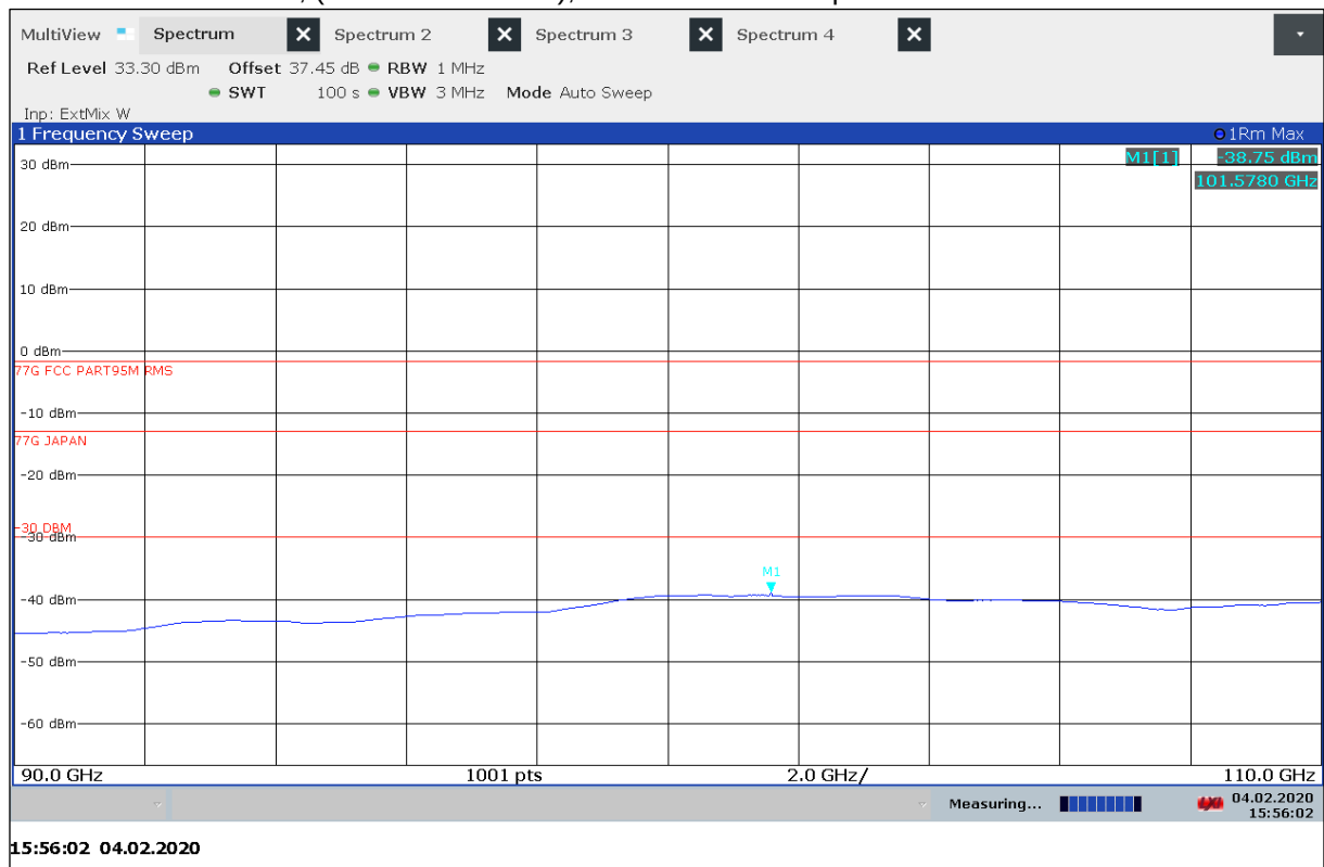
Plot 28: 90 GHz – 110 GHz, (valid for all modes), vertical / horizontal polarization
