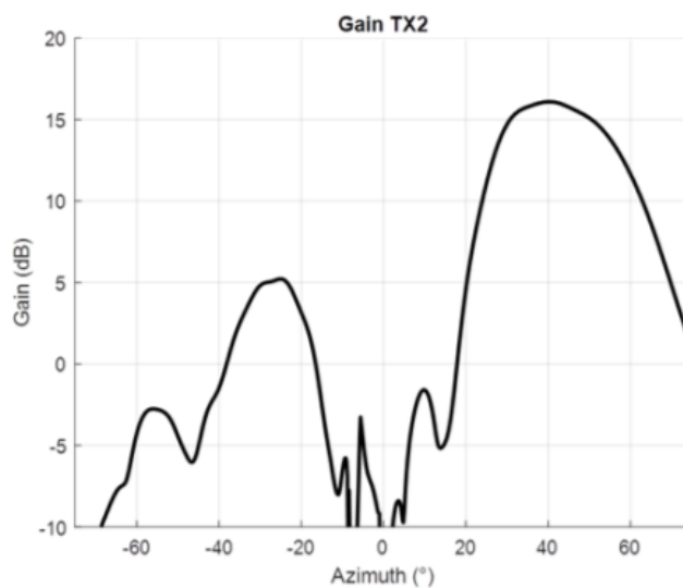
Figure 7: CR5CPCCF TX2 antenna characteristics
