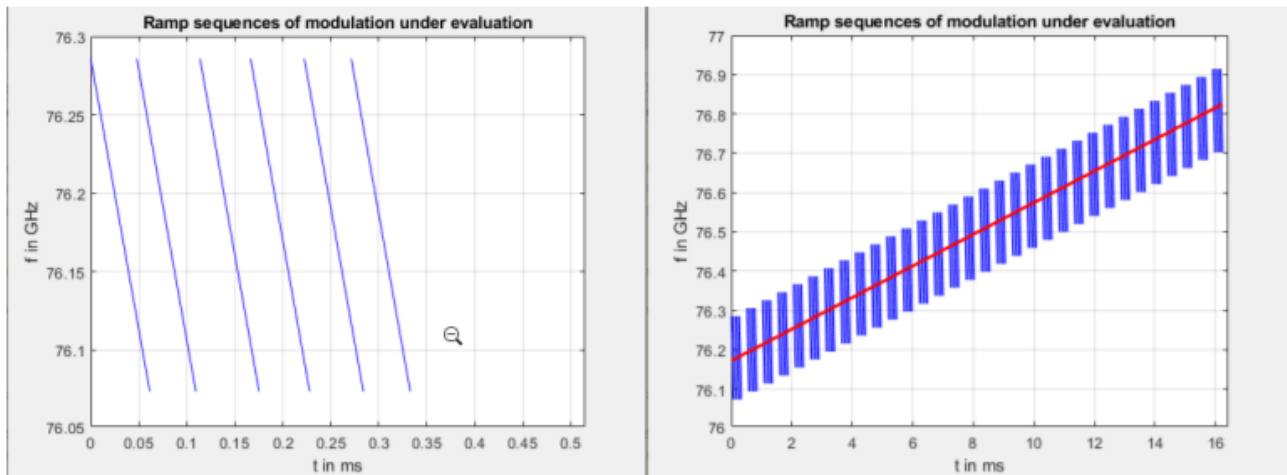
Figure 12: DMP07 single sequence and complete burst.
