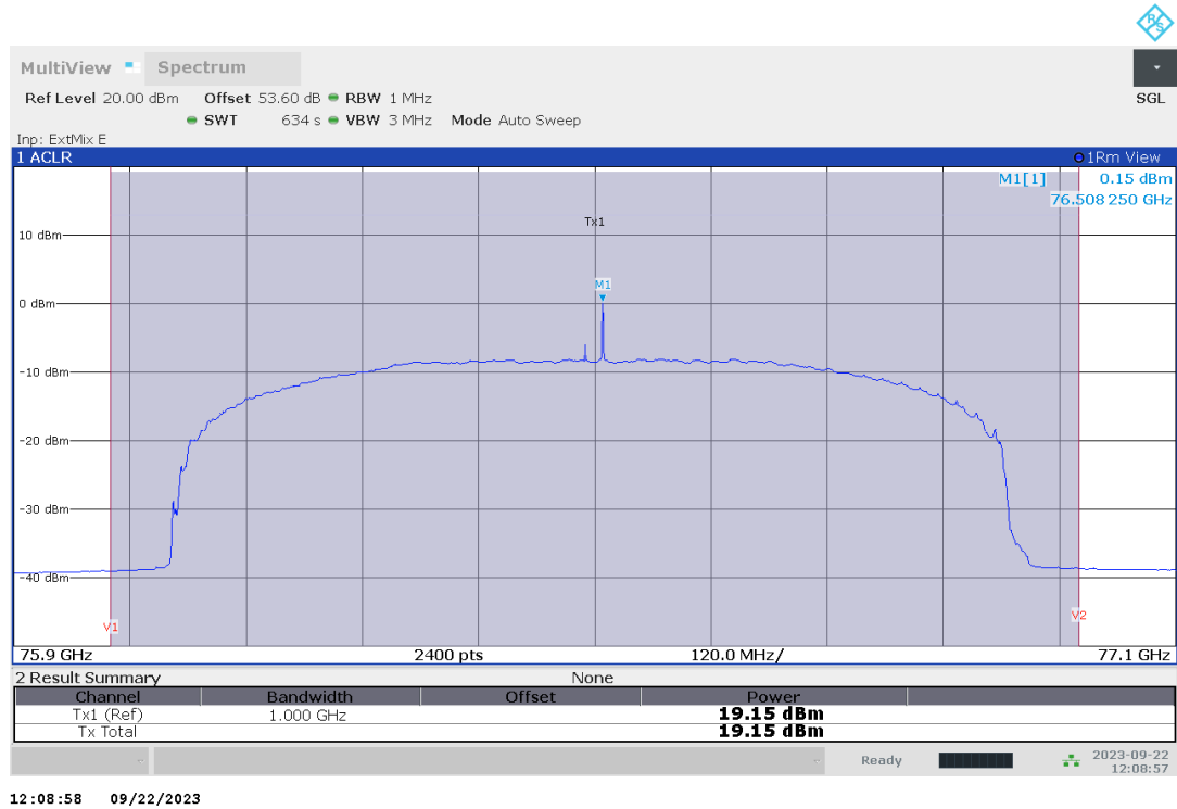
Plot no. 1: Mean Power EIRP, RMS detector / Channel Power, EUT Mode 7
