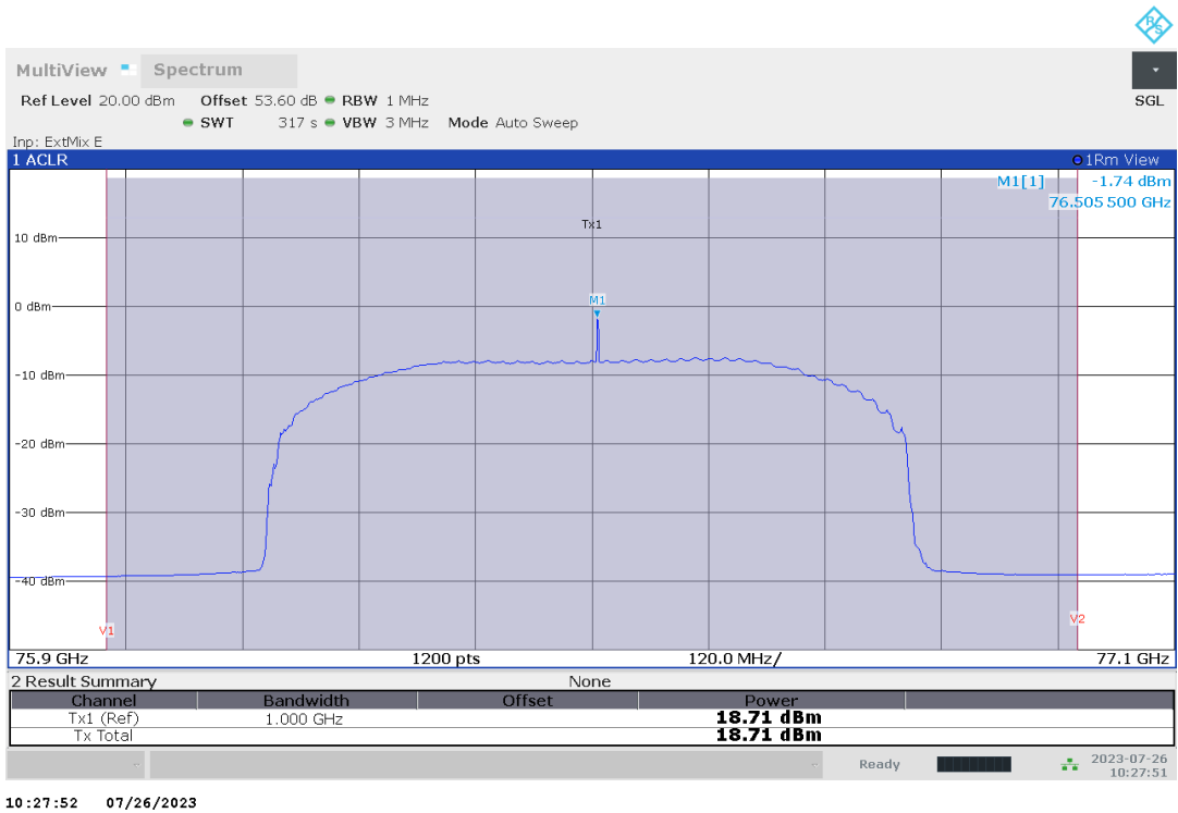
Plot no. 3: Mean Power EIRP, RMS detector / Channel Power, EUT Mode 9
