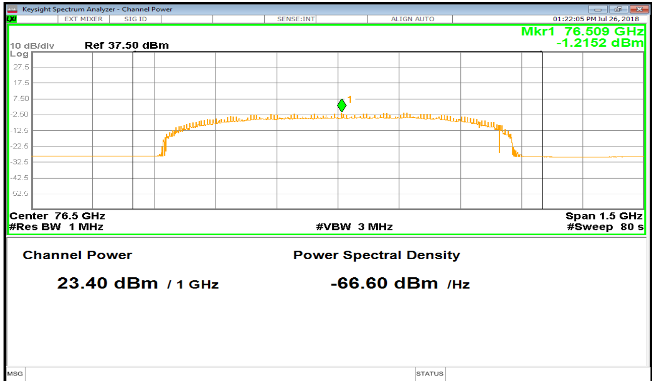
Plot 5: Radiated mean power, T_{\min} / V_{\text{nom}}
