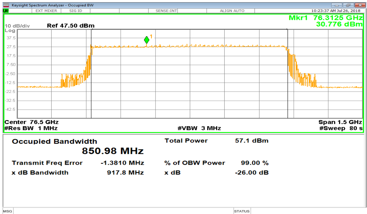
Plot 1: OBW, Radiated peak power, T_{\text{nom}} / V_{\text{min-max}}
