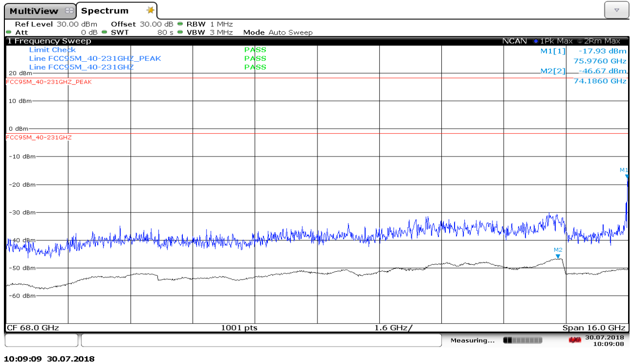
Plot 15: 60 GHz to 76 GHz
