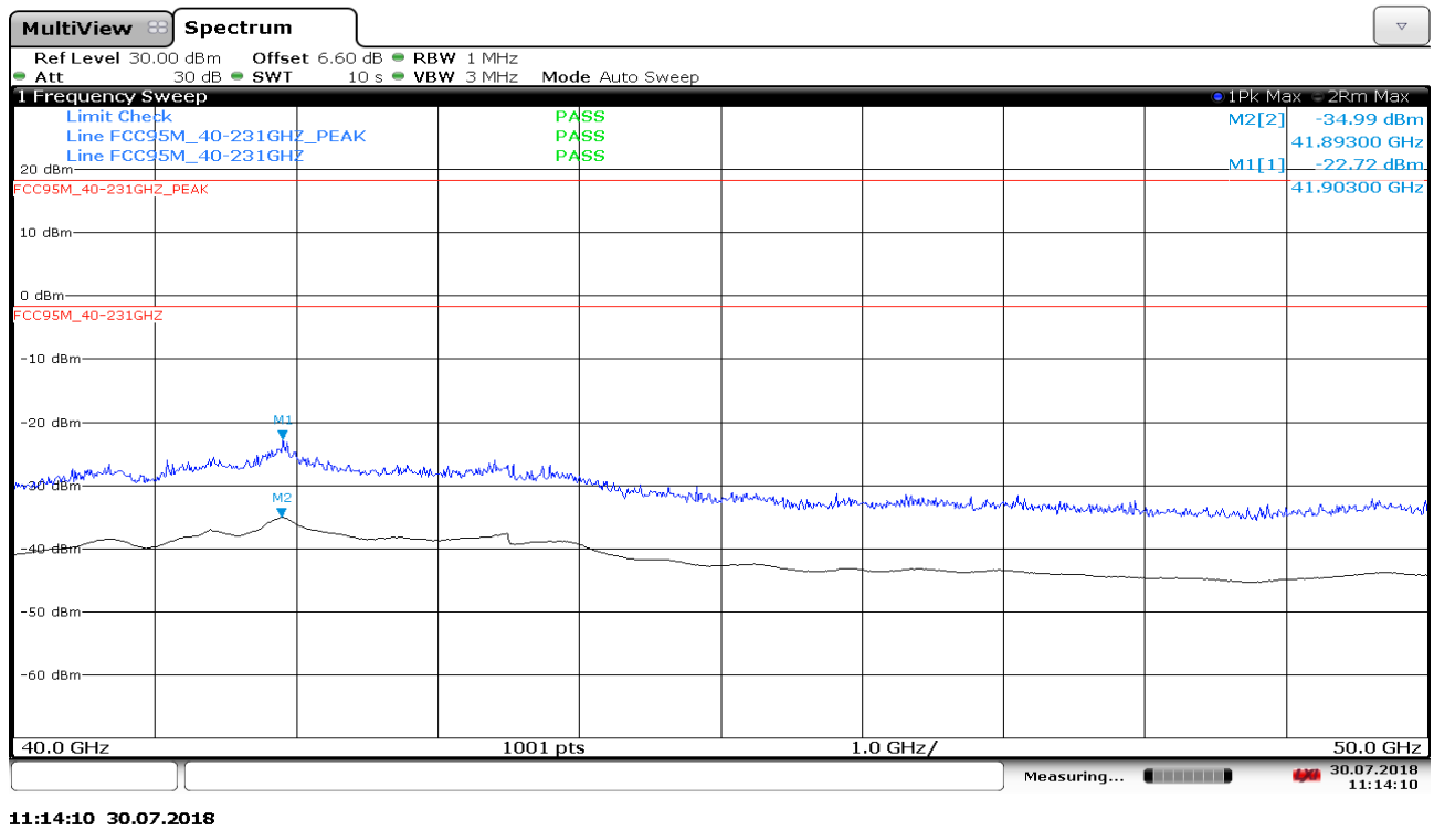
Plot 13: 40 GHz to 50 GHz
