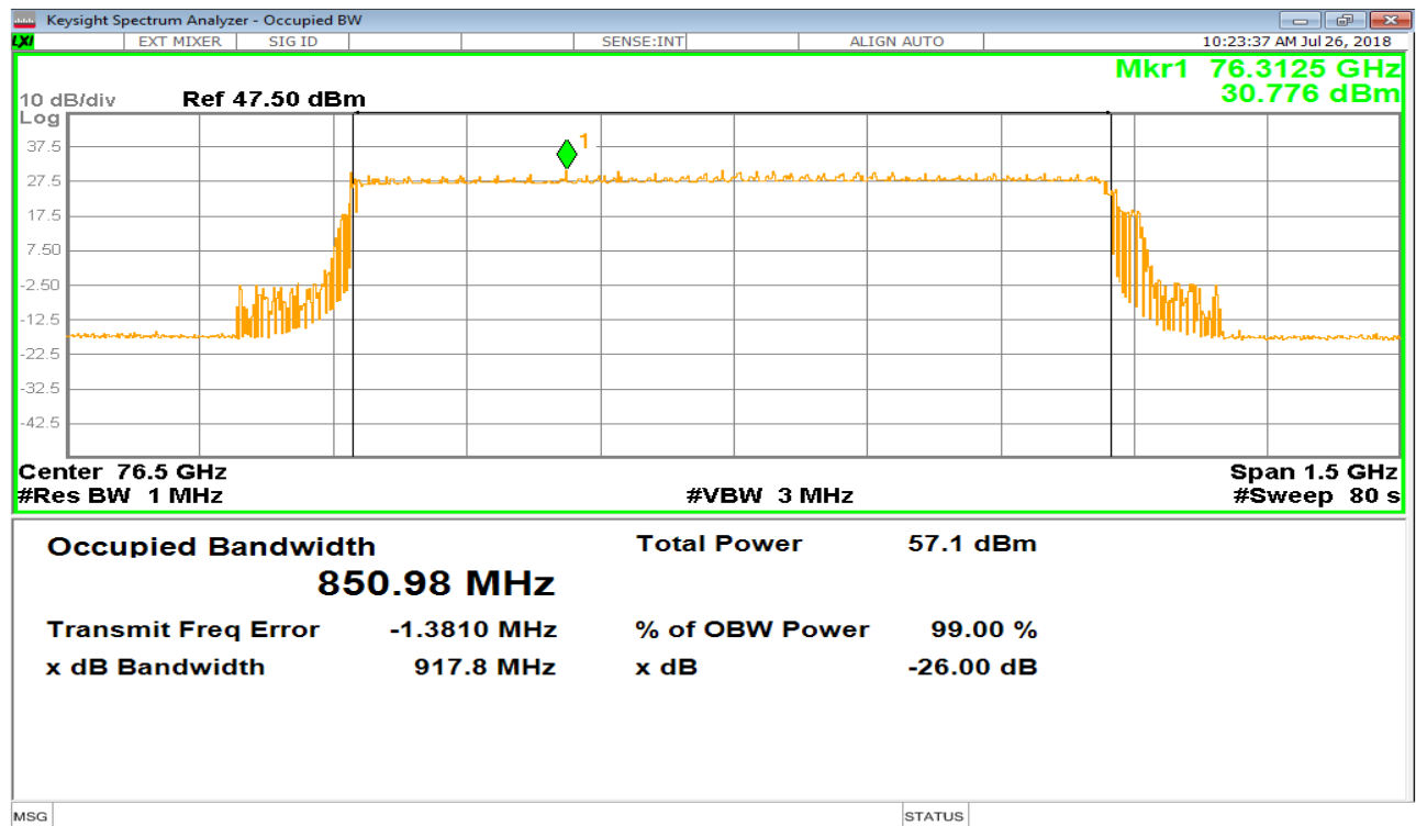
Plot 28: OBW mode 7, 20 °C
