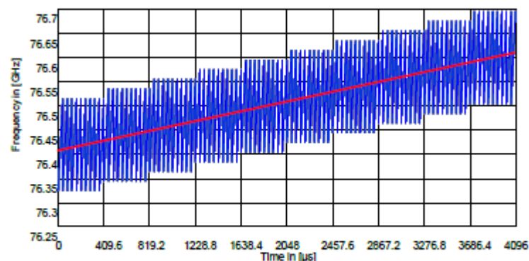
Figure 5 Example one chirp sequence out of 10 sequences
