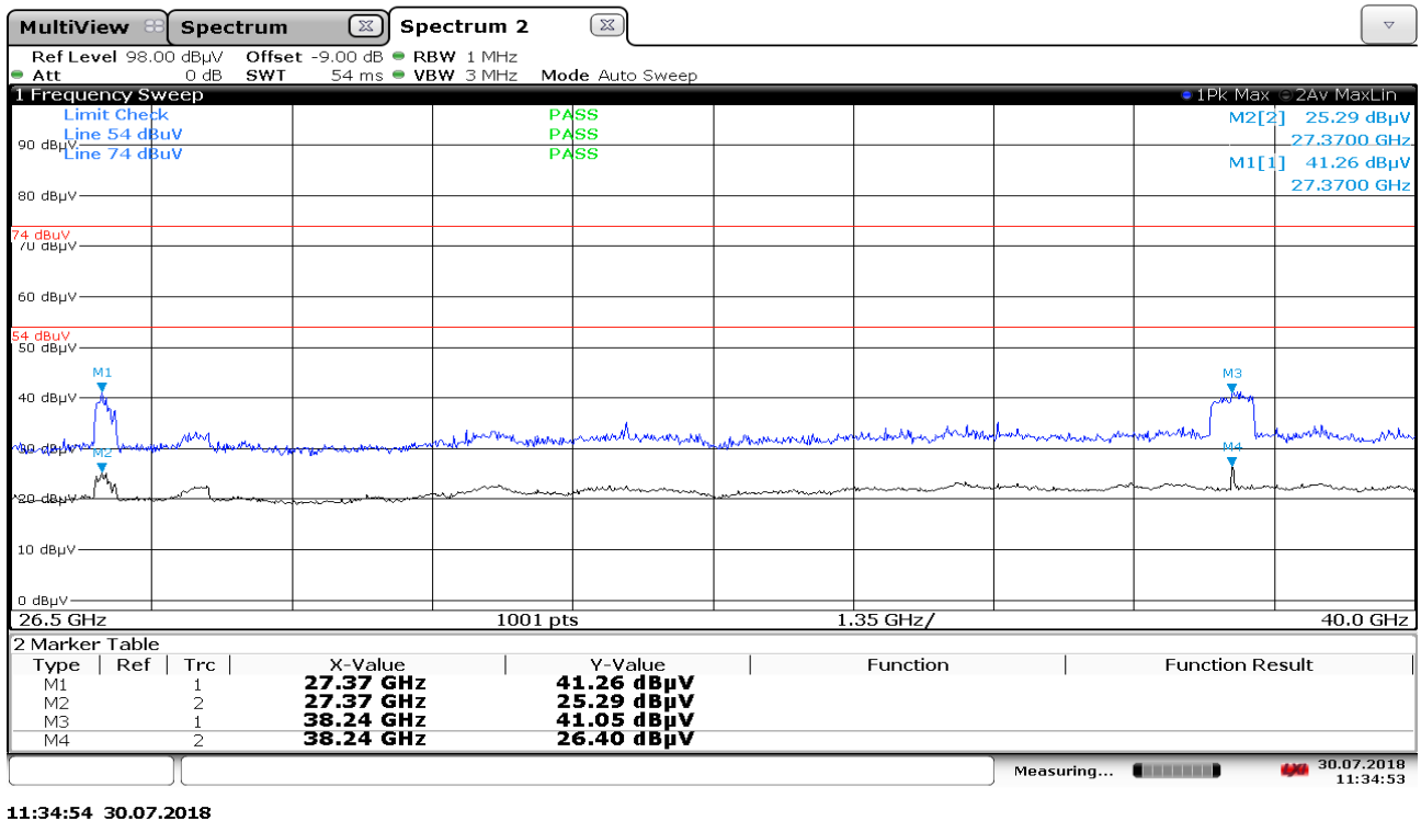
Plot 12: 26 GHz to 40 GHz
