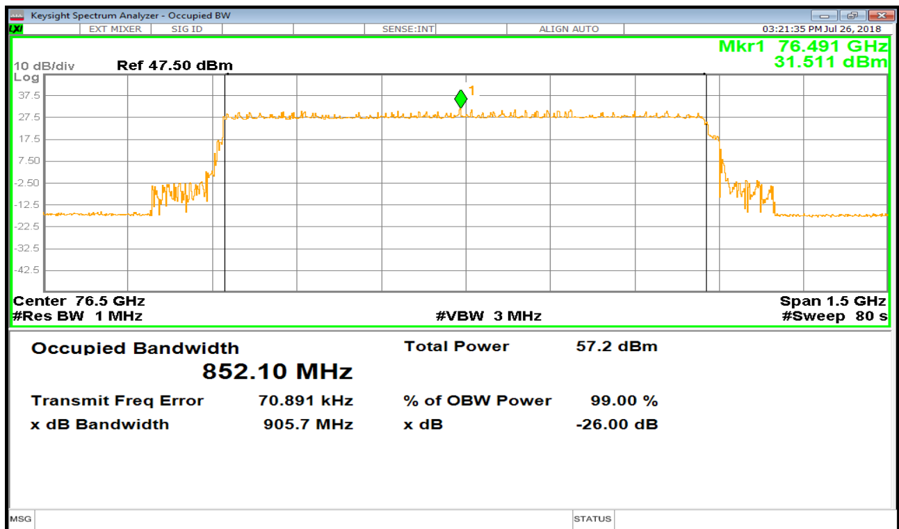
Plot 3: OBW, Radiated peak power, T_{\max} / V_{\text{nom}}
