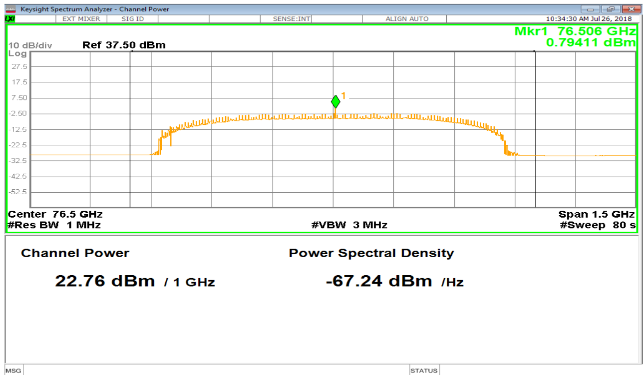
Plot 4: Radiated mean power, T_{\text{nom}} / V_{\text{min-max}}
