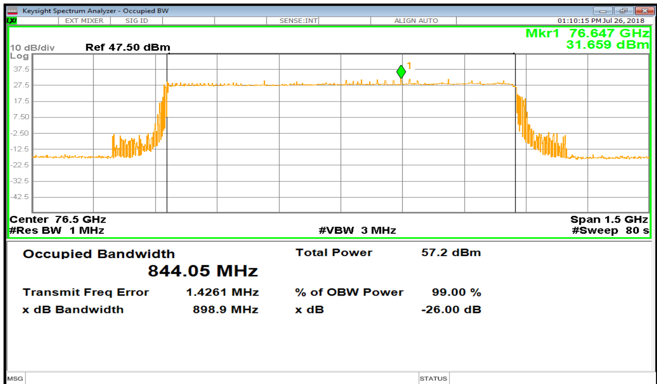
Plot 2: OBW, Radiated peak power, T_{\text{min}} / V_{\text{nom}}
