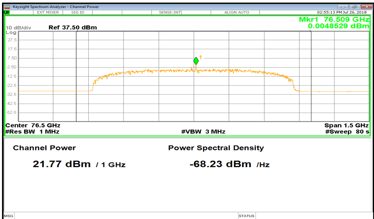
Plot 6: Radiated mean power, T_{\max} / V_{\text{nom}}
