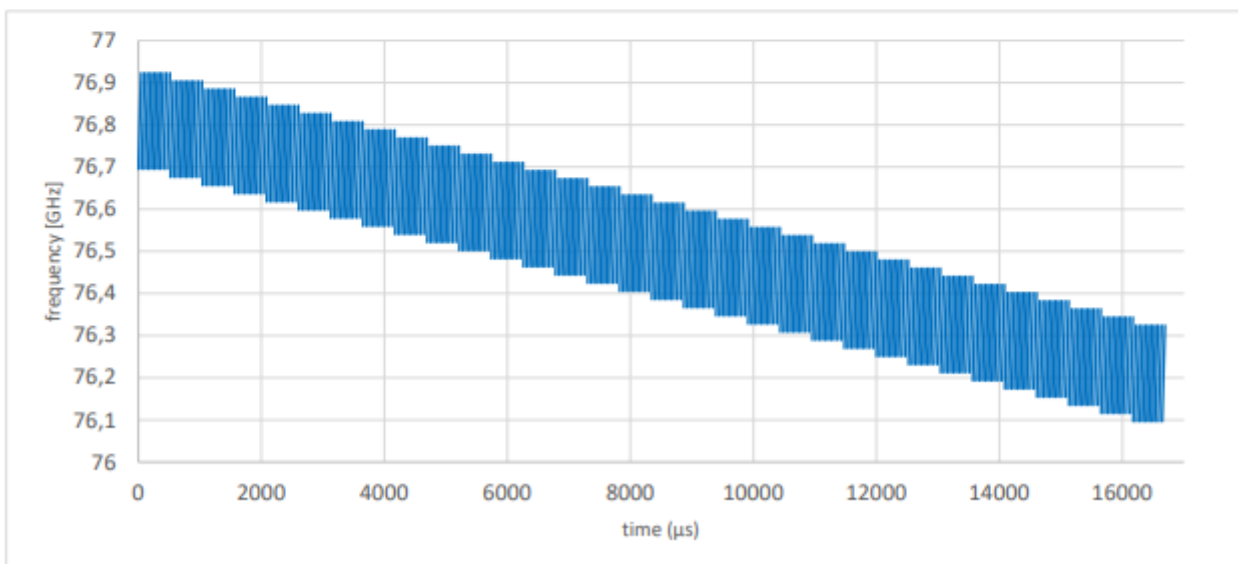
Figure 7: Single burst
