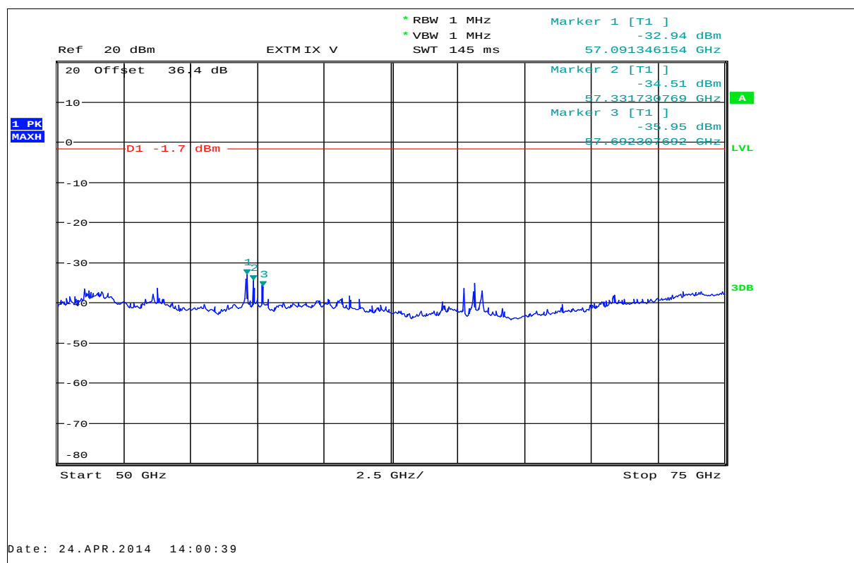
Plot 18: 50 GHz – 75 GHz, antenna horizontal and vertical, low / mid / high frequency
