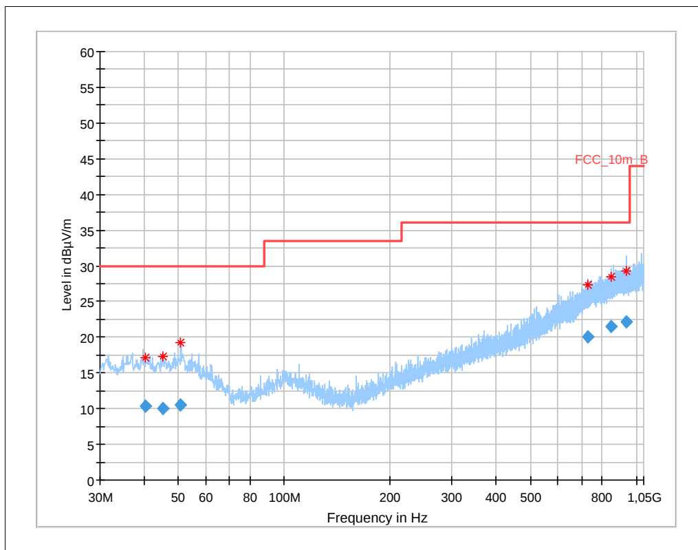
Plot 8: 30 MHz – 1 GHz, antenna horizontal and vertical, low frequency
