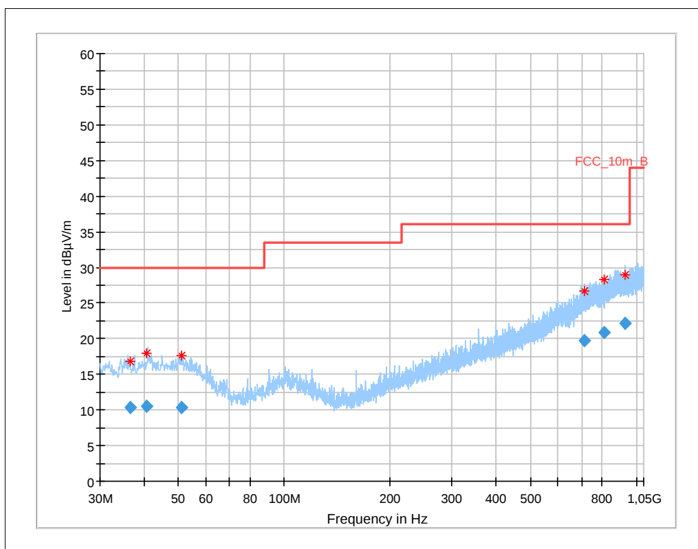
Plot 9: 30 MHz – 1 GHz, antenna horizontal and vertical, mid frequency
