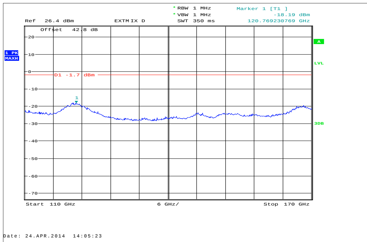
Plot 20: 110 GHz – 170 GHz, antenna horizontal and vertical, low / mid / high frequency
