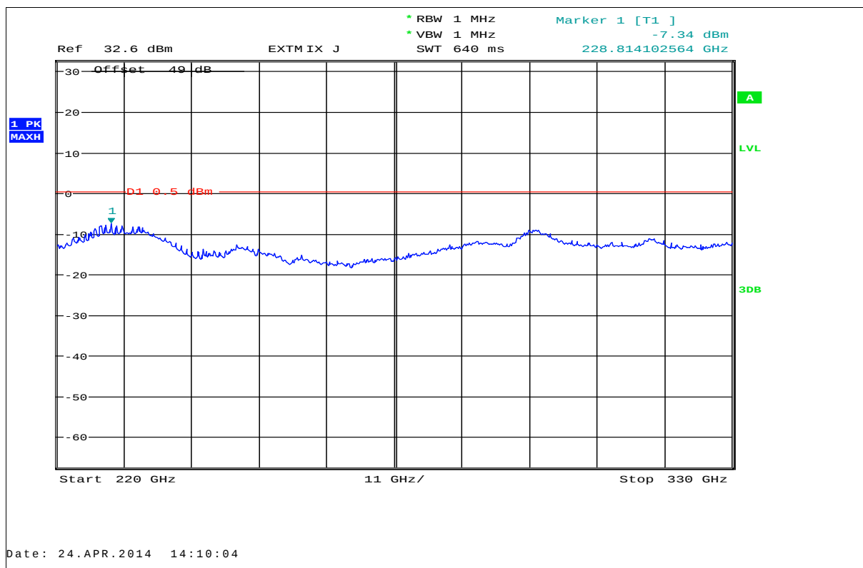
Plot 22: 220 GHz – 330 GHz, antenna horizontal and vertical, low / mid / high frequency
