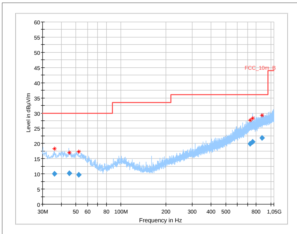
Plot 10: 30 MHz – 1 GHz, antenna horizontal and vertical, high frequency
