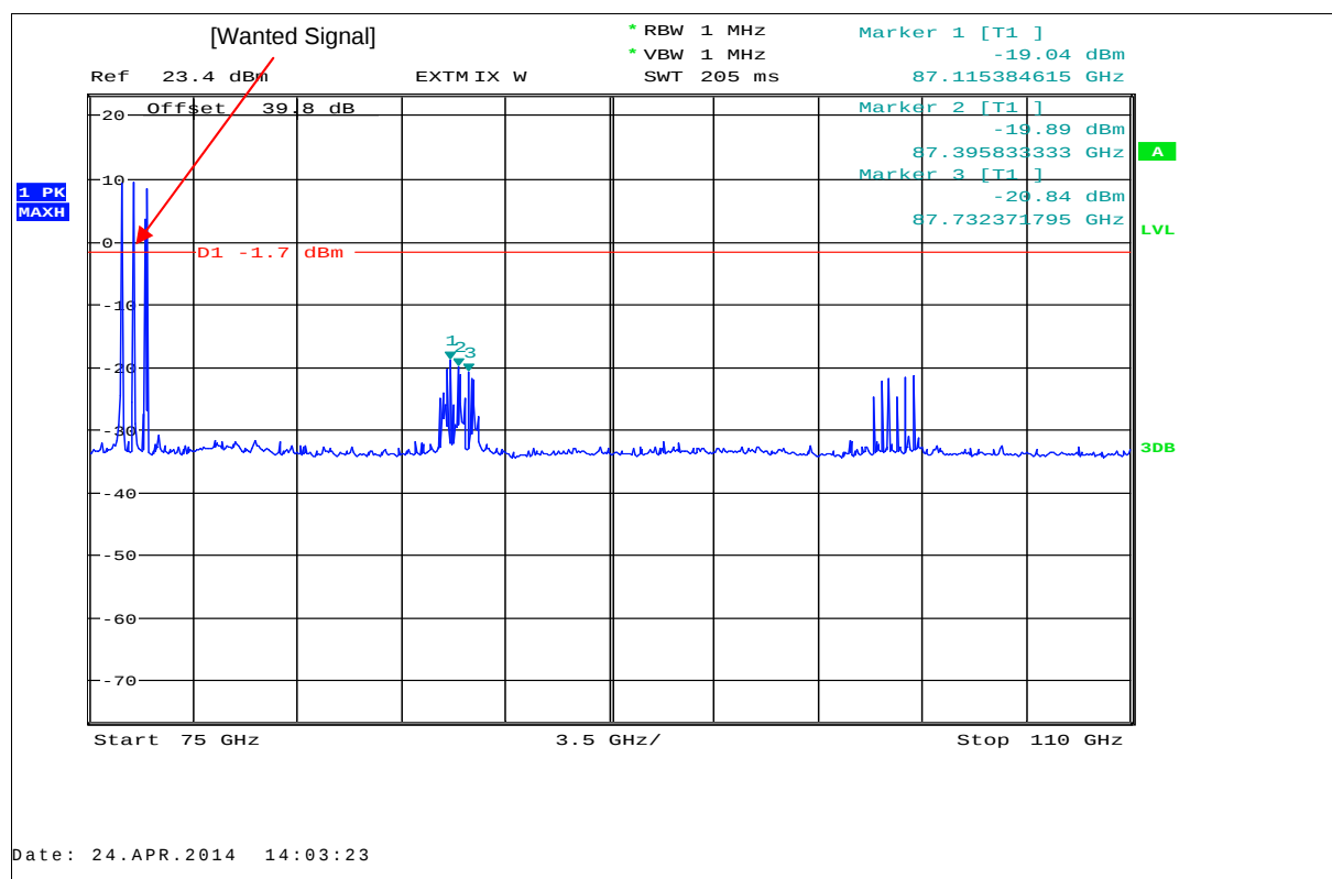
Plot 19: 75 GHz – 110 GHz, antenna horizontal and vertical, low / mid / high frequency
