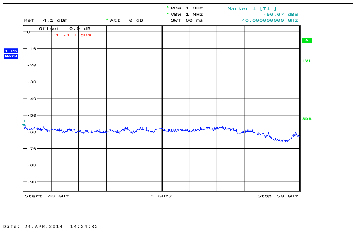
Plot 17: 40 GHz – 50 GHz, antenna horizontal and vertical, low / mid / high frequency
