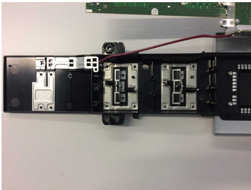
Antenna assembly 2 detail view
