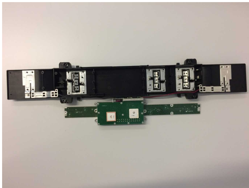
Antenna assembly 1 overview
