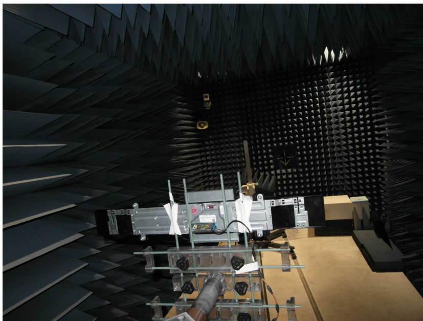
setup OTA antenna 2
