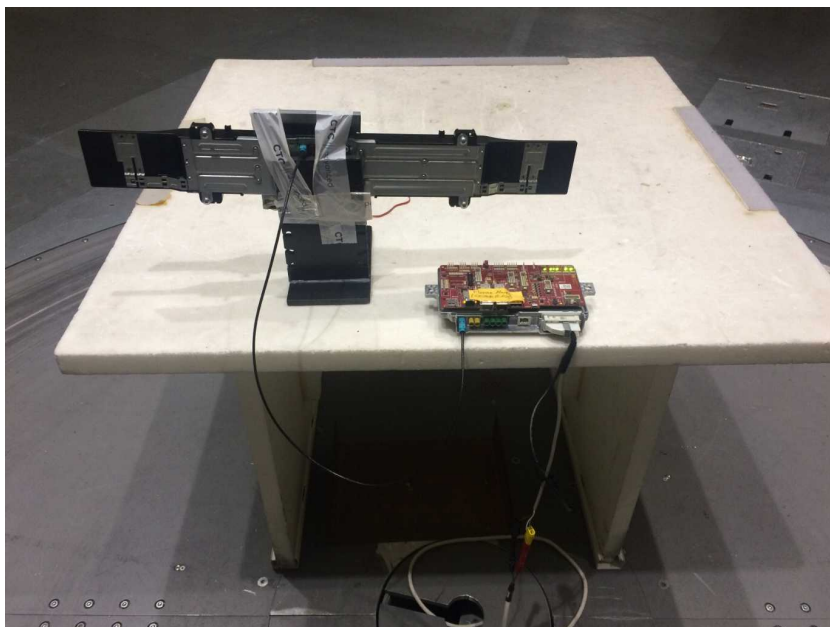
RSE setup < 1GHz antenna 2
