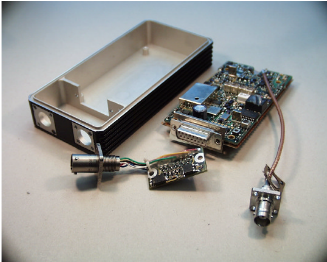
Fig. 3 : Electronics and Housing
