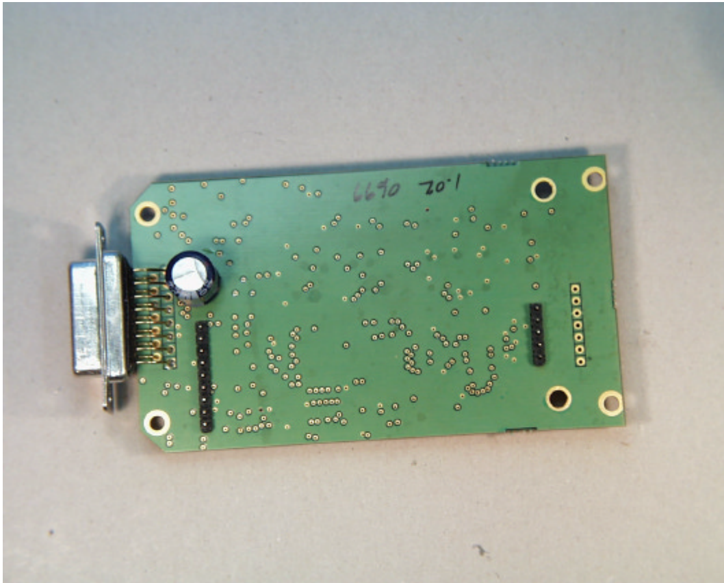
Fig. 5 : Logic PCB, Top View (identical to Sateline 3AS)
