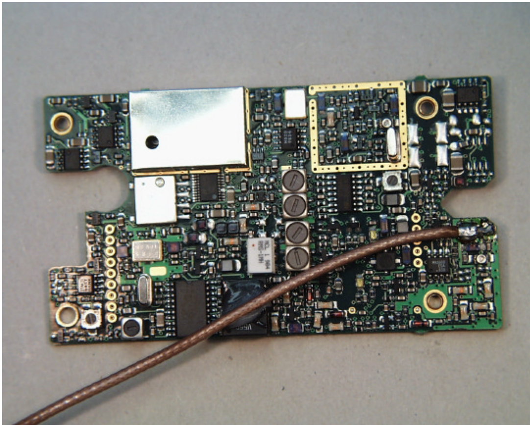
Fig. 7 : RF PCB, Top View (identical to Sateline 3AS)
