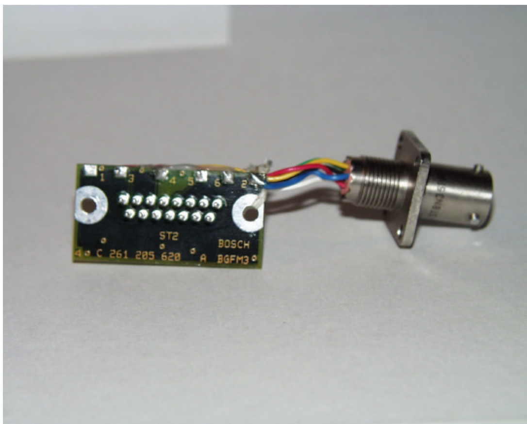
Fig. 10 : Adaptor Board, Bottom View
