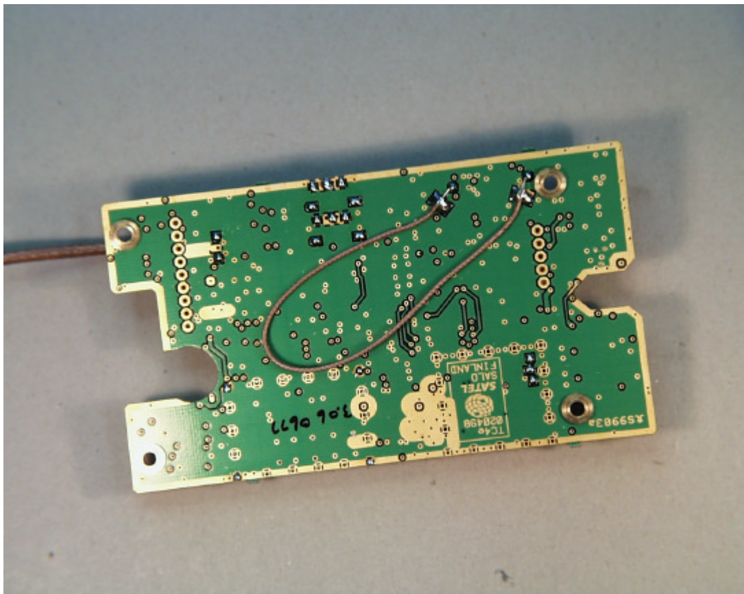
Fig. 8 : RF PCB, Bottom View (identical to Sateline 3AS)
