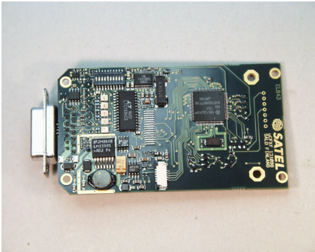
Fig. 6 : Logic PCB, Bottom View (identical to Sateline 3AS)
