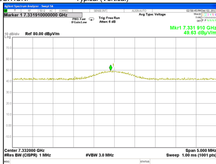
Plot 7.2.20 Radiated emission measurements at the eighth harmonic frequency
