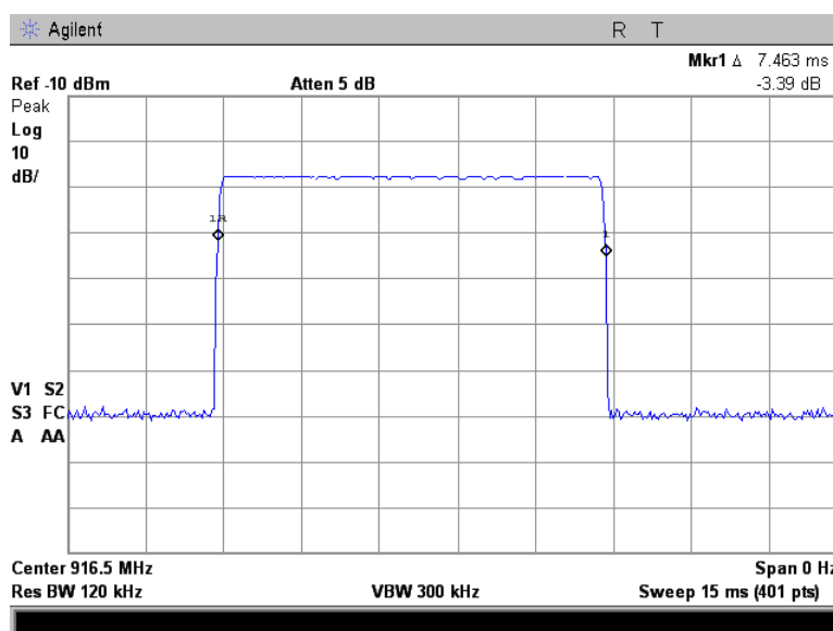
Plot 7.2.26 Supervision transmission period
