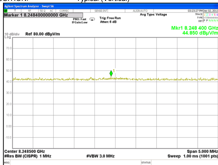
Plot 7.2.22 Radiated emission measurements at the ninth harmonic frequency
