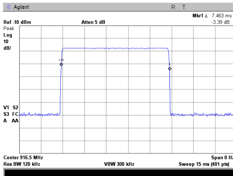
Plot 7.1.2 Supervision transmission duration
