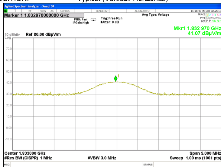
Plot 7.2.10 Radiated emission measurements at the second harmonic frequency
