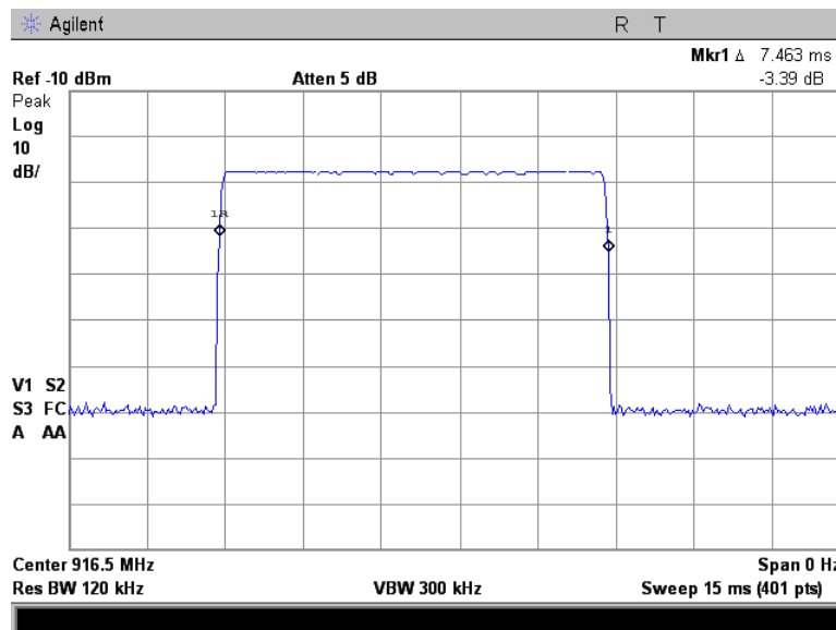
Plot 7.2.27 Supervision transmission duration
