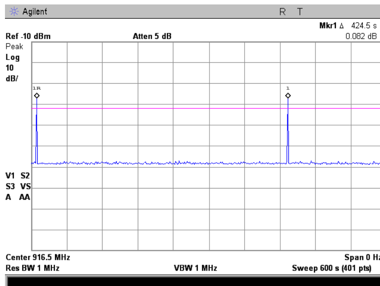
Plot 7.2.28 Supervision transmission period
