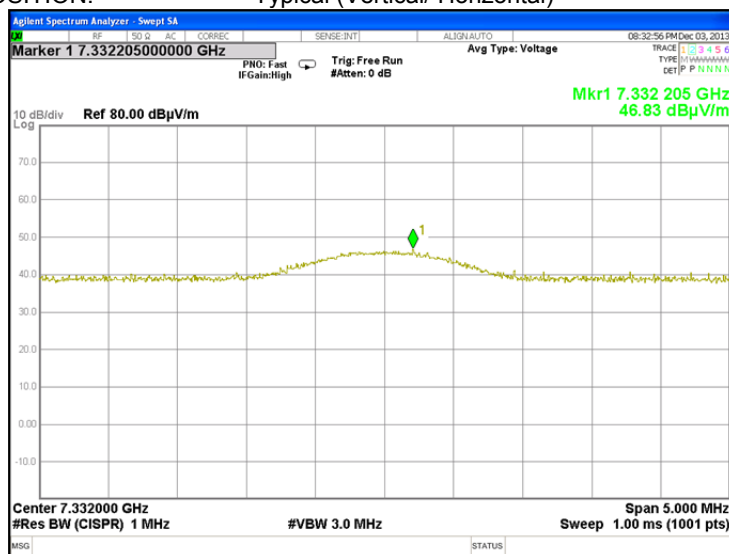
Plot 7.2.22 Radiated emission measurements at the eighth harmonic frequency
