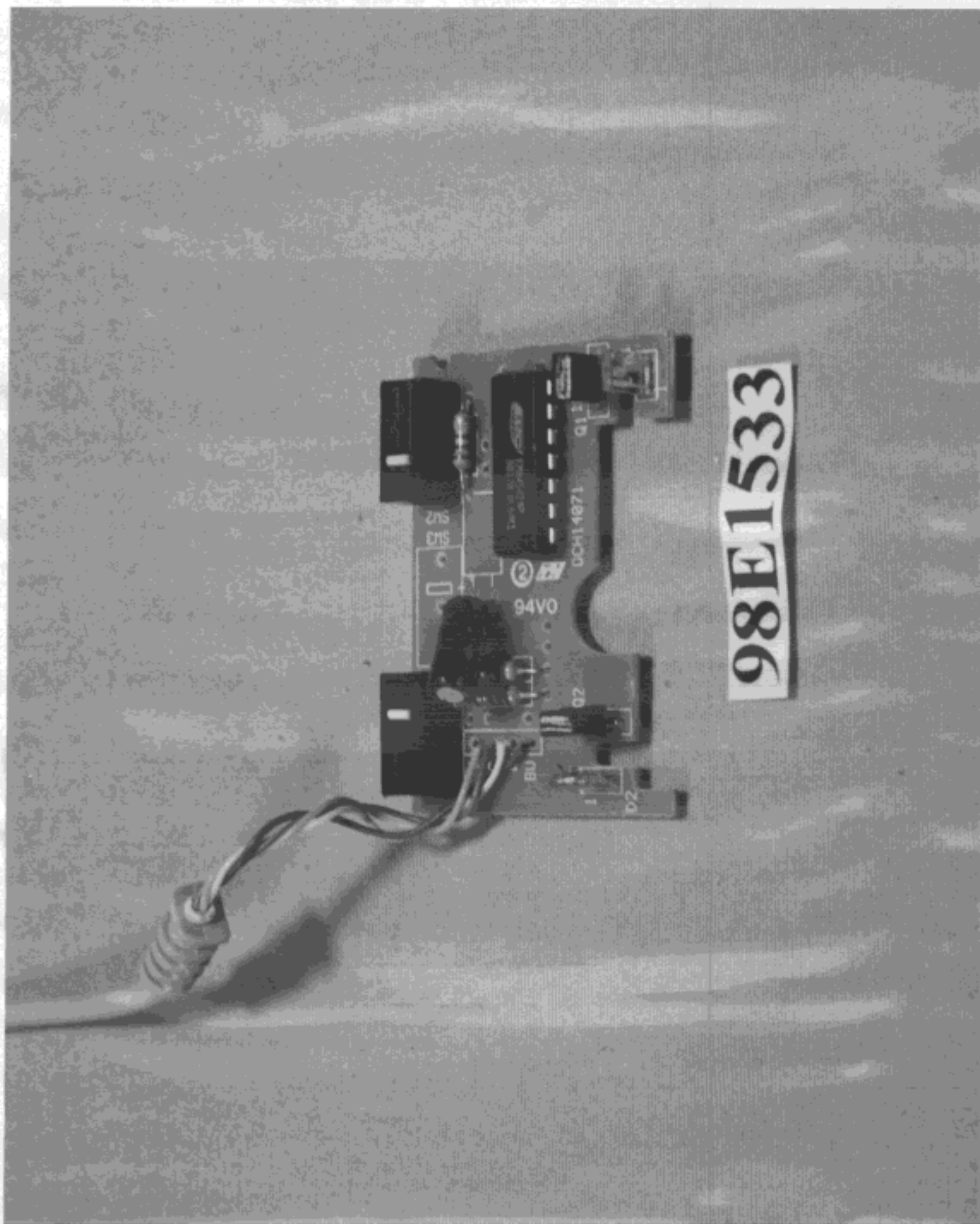
Photo # 10. SP3000 Unit Partially Disassembled
