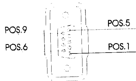
SR2000/SR3000 9 Pin D-subminiature Connector
