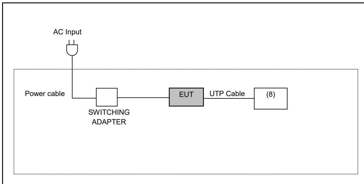
Radiated Emission
