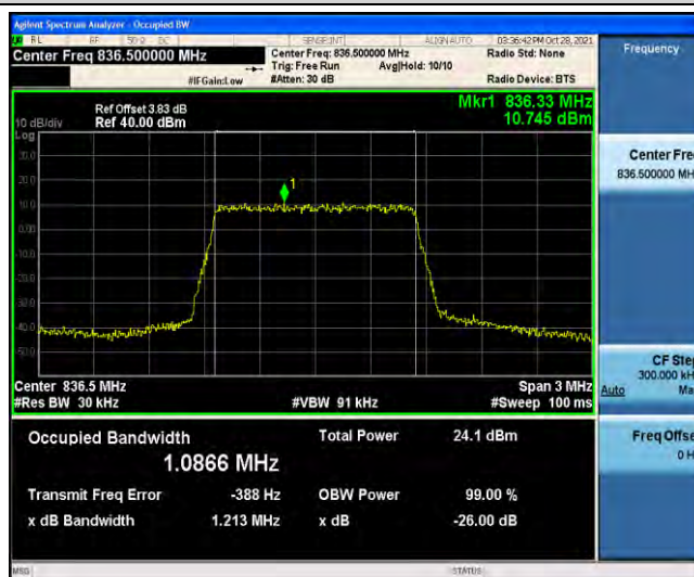
Band5-1.4MHz-QPSK-20525-6RB#0-1.0866
