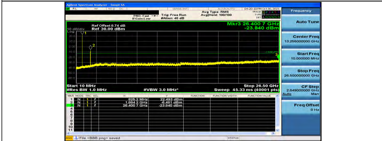
(Channel Bandwidth: 10 MHz)_LCH_ DFT-s Pi/2 BPSK_1RB#0
