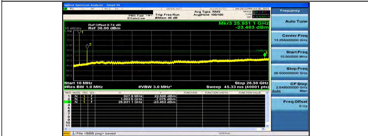
(Channel Bandwidth: 20 MHz)_MCH_ DFT-s Pi/2 BPSK_1RB#0
