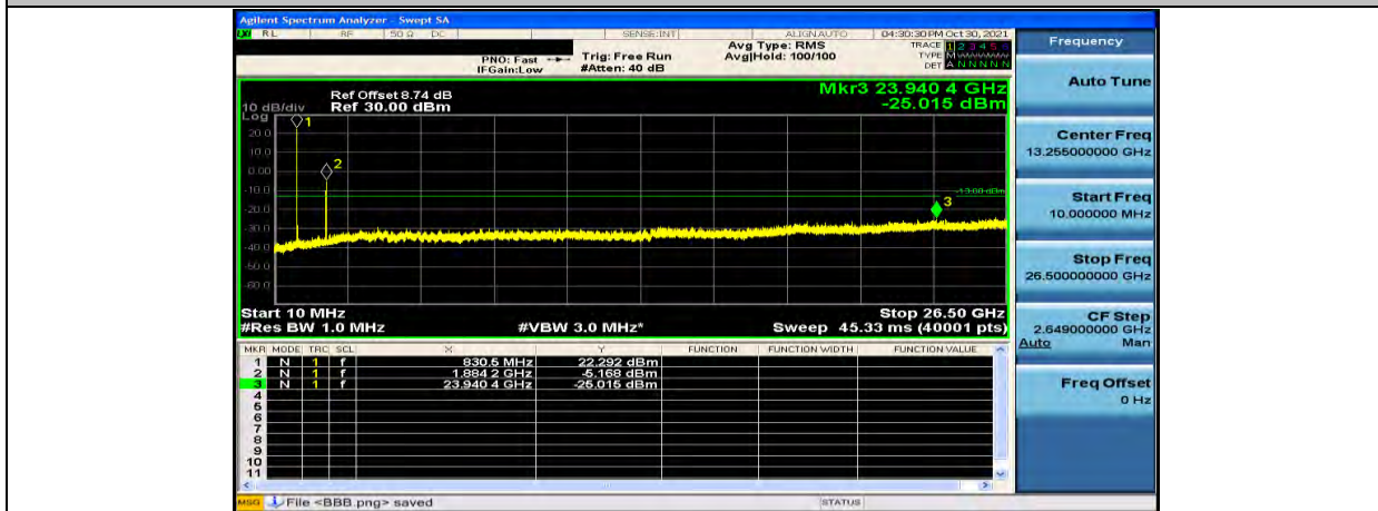
(Channel Bandwidth: 20 MHz)_HCH_ DFT-s Pi/2 BPSK_1RB#0
