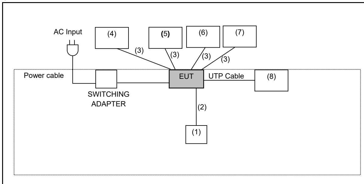
Conducted Emissions
