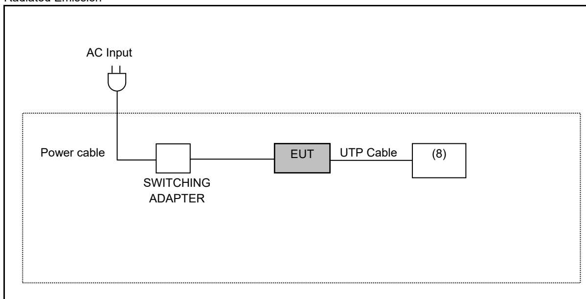
Radiated Emission
