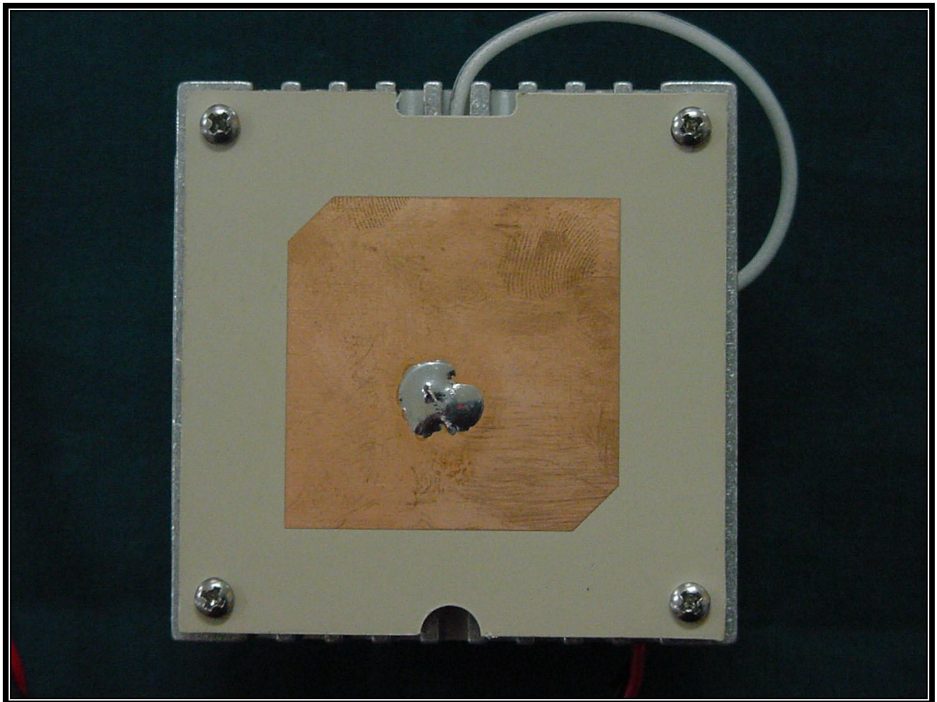
PHOTOGRAPH 5: ANTENNA FRONT VIEW
