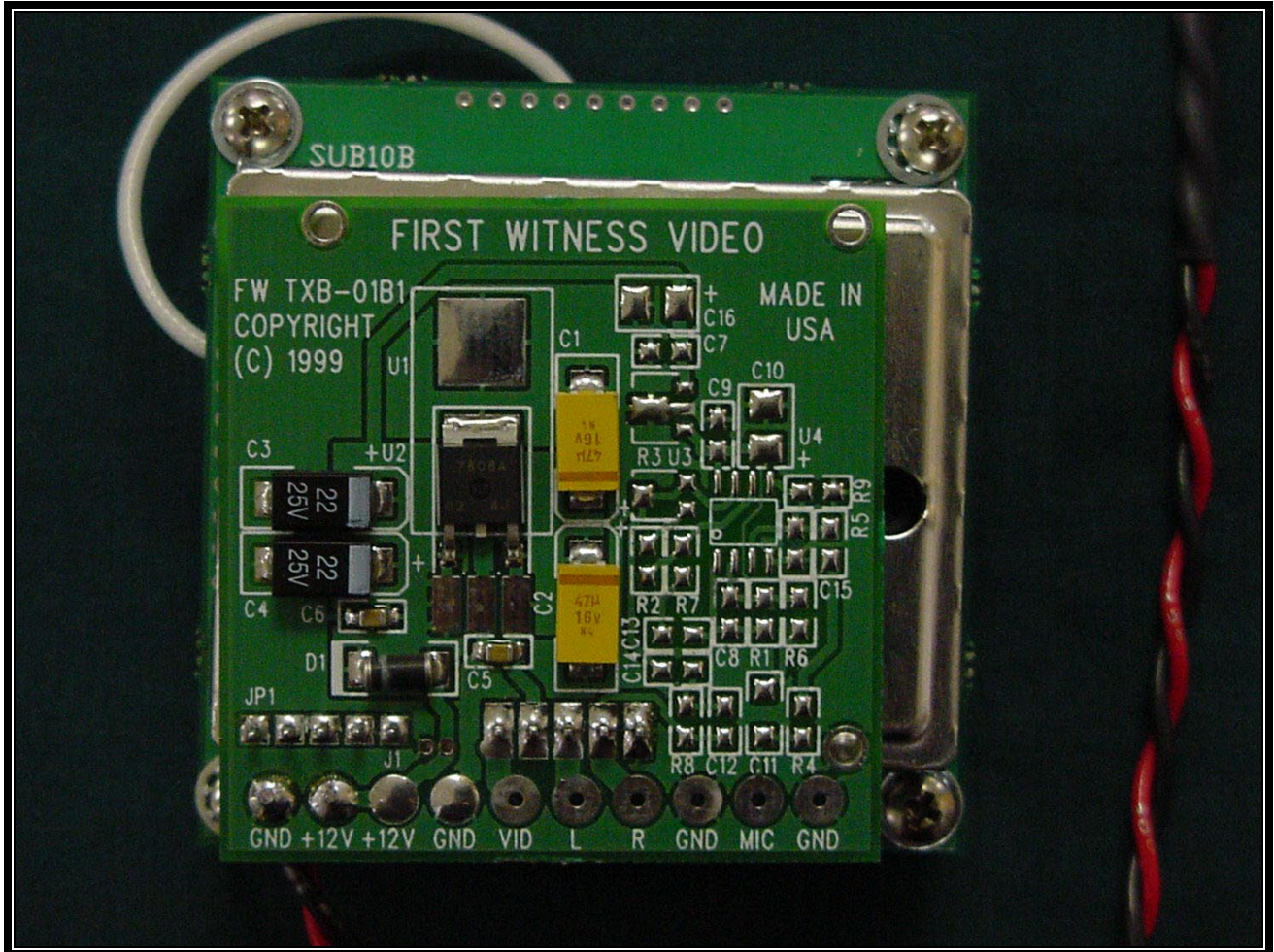
PHOTOGRAPH 3: RF MODULE FRONT VIEW
