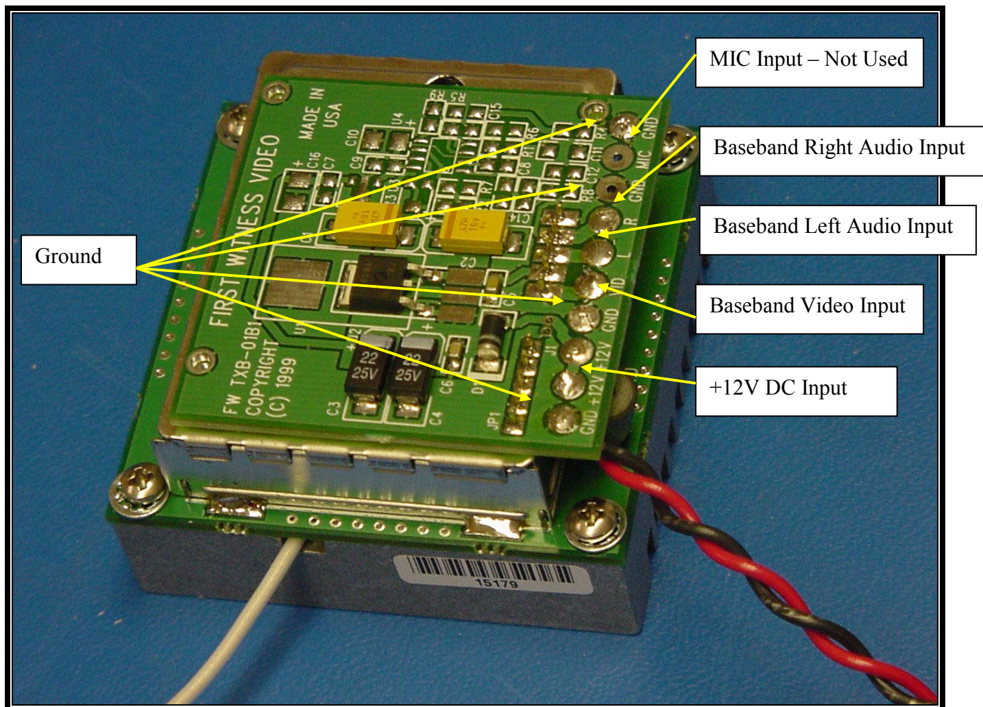
PHOTOGRAPH 4: DETAILED EUT VIEW
