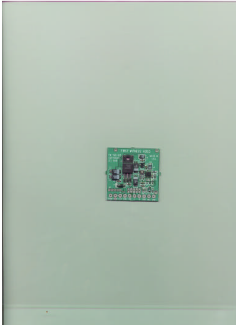
Figure 7: Power/Amp PCB Board, Component Side
