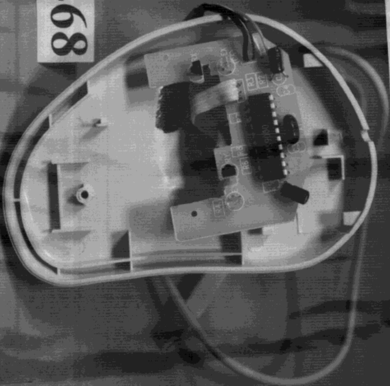
Photo # 4. Unit Partially Disassembled
