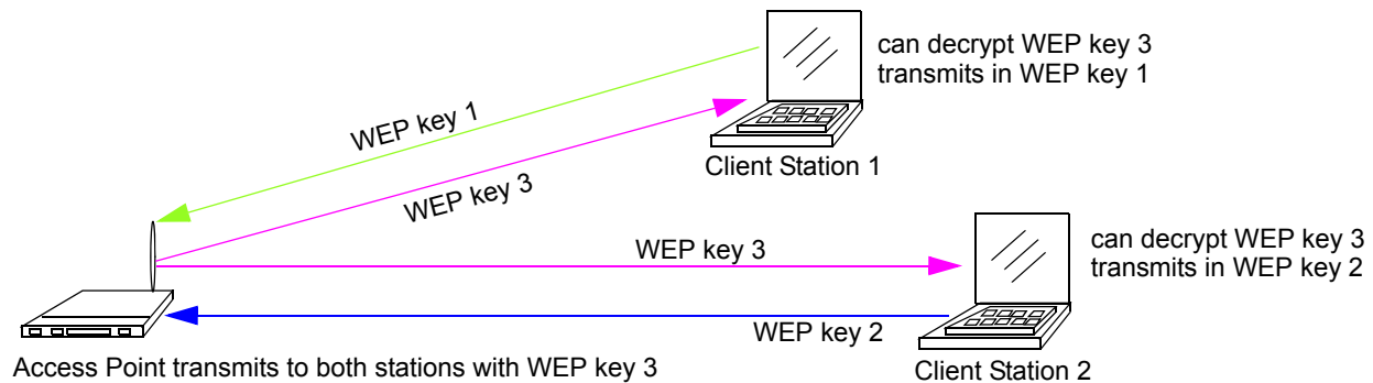
Figure 9. Example of Using Multiple WEP Keys and Transfer Key Index on Client Devices
