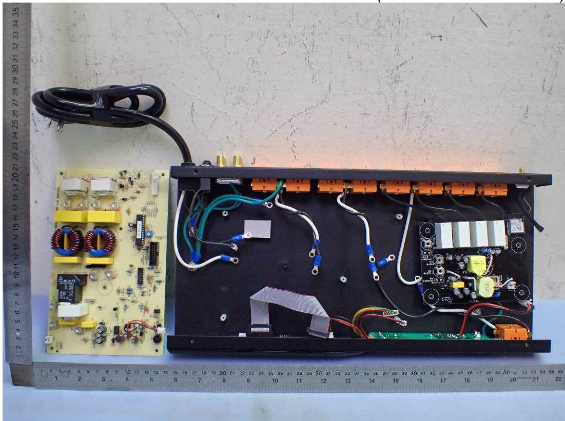
Figure 8 Internal View (Removed Internal Board)
