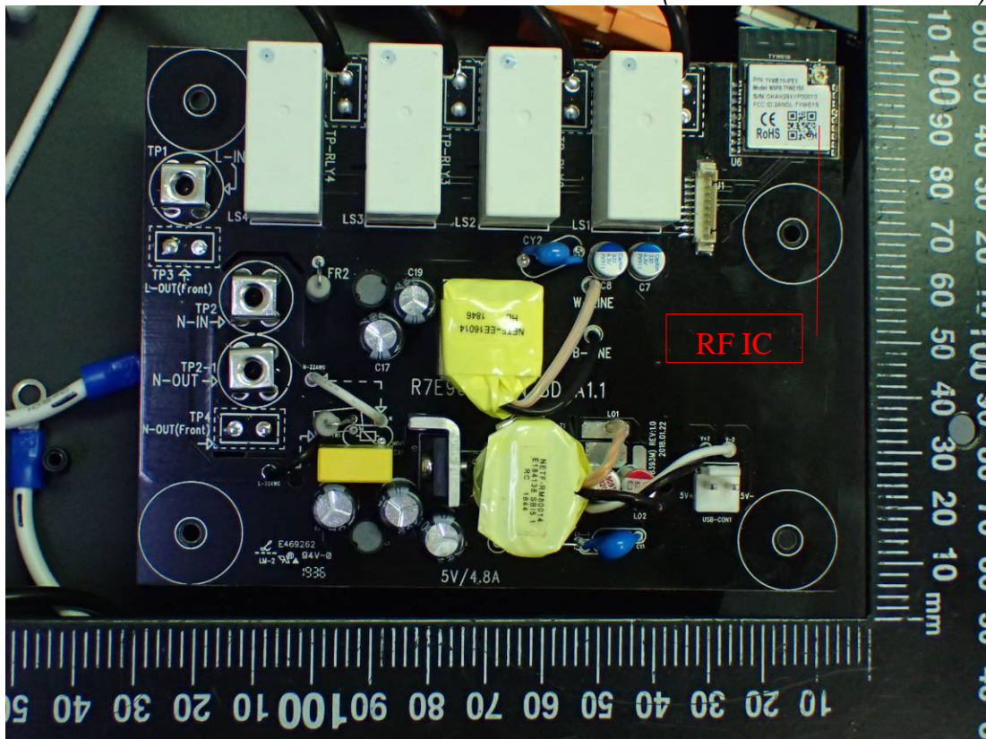
Figure 13 Internal View (Main Board / Front View)
