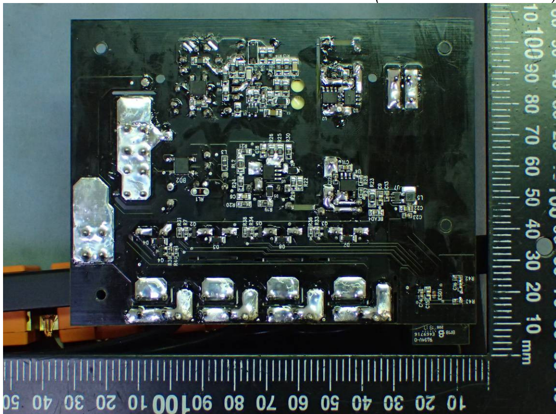
Figure 14 Internal View (Main Board / Back View)
