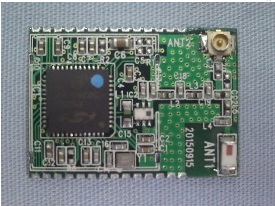
Figure 4 Internal View
