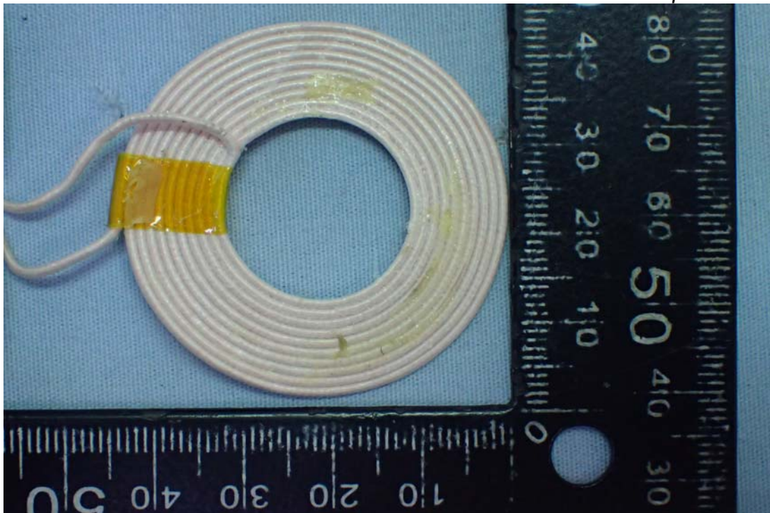
Figure 6 Loop Antenna
