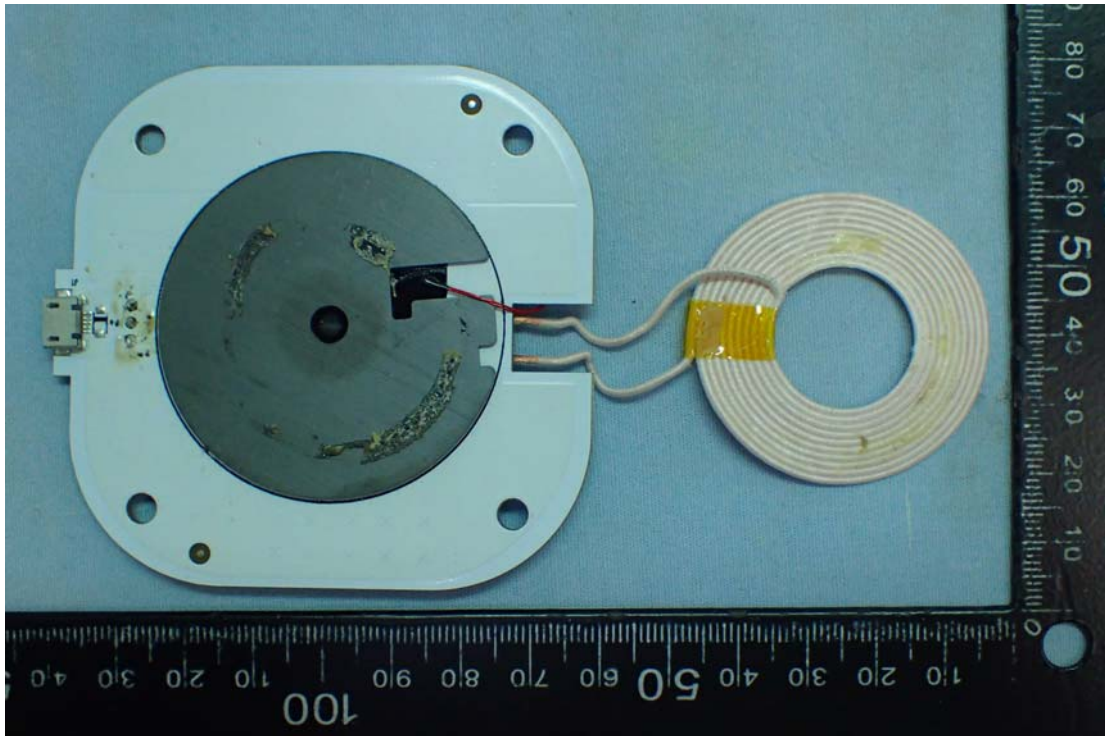
Figure 5 Internal View
