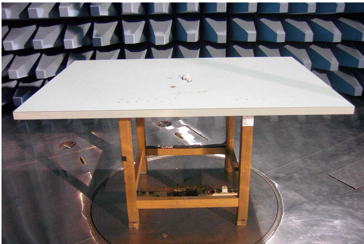
The Test Configuration of X-plane
