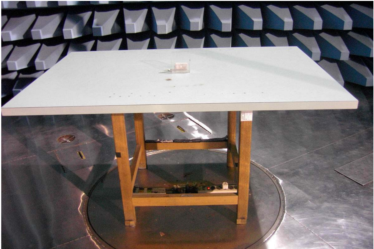
The Test Configuration of Z- plane
