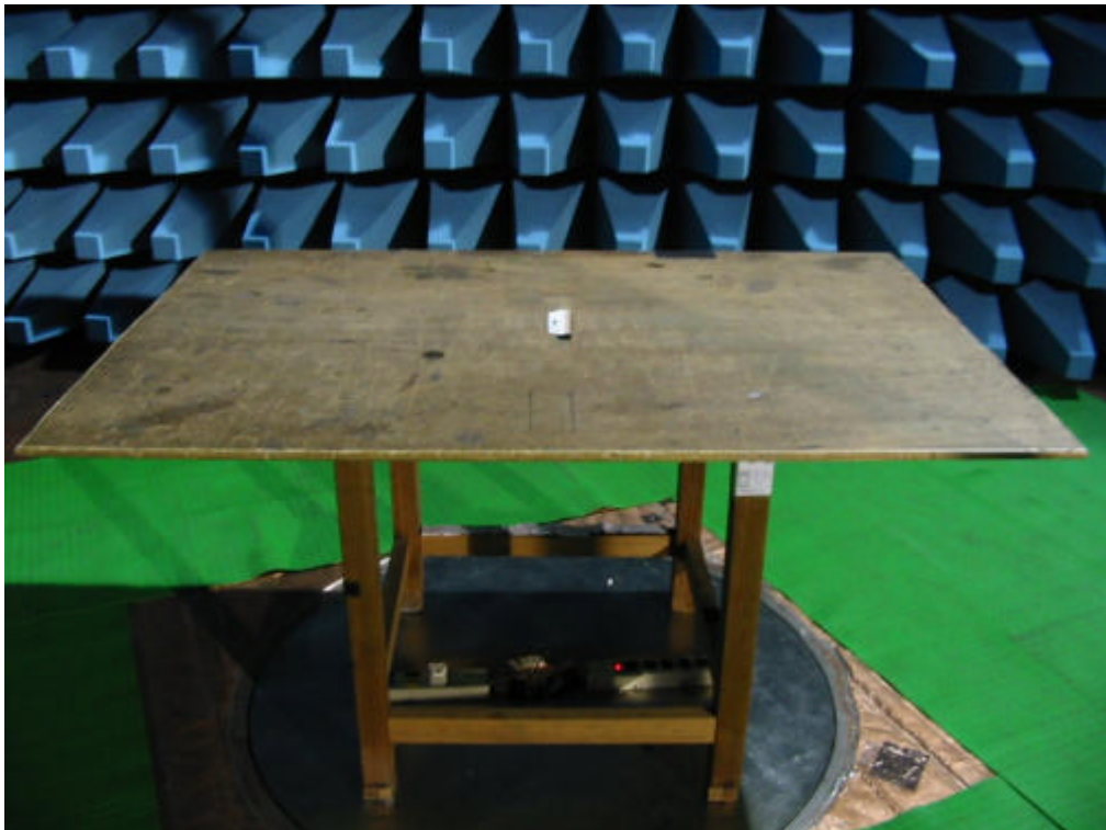
Front View of Y-axis
