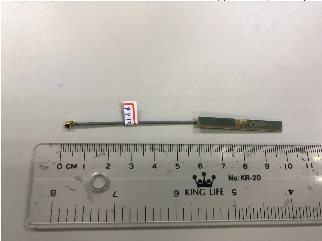
Figure 3 General Appearance (Antenna, Back View)
