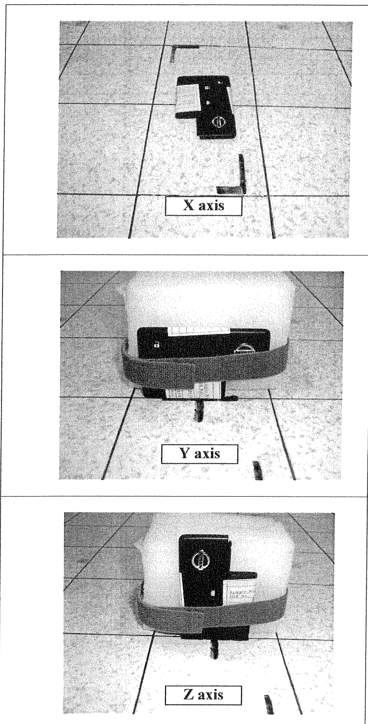
Worse case X axis (Measurement Biconical antenna Polarization :Horizontal) And Worst case Z axis (Measurement Biconical antenna Polarization: Vertical)
