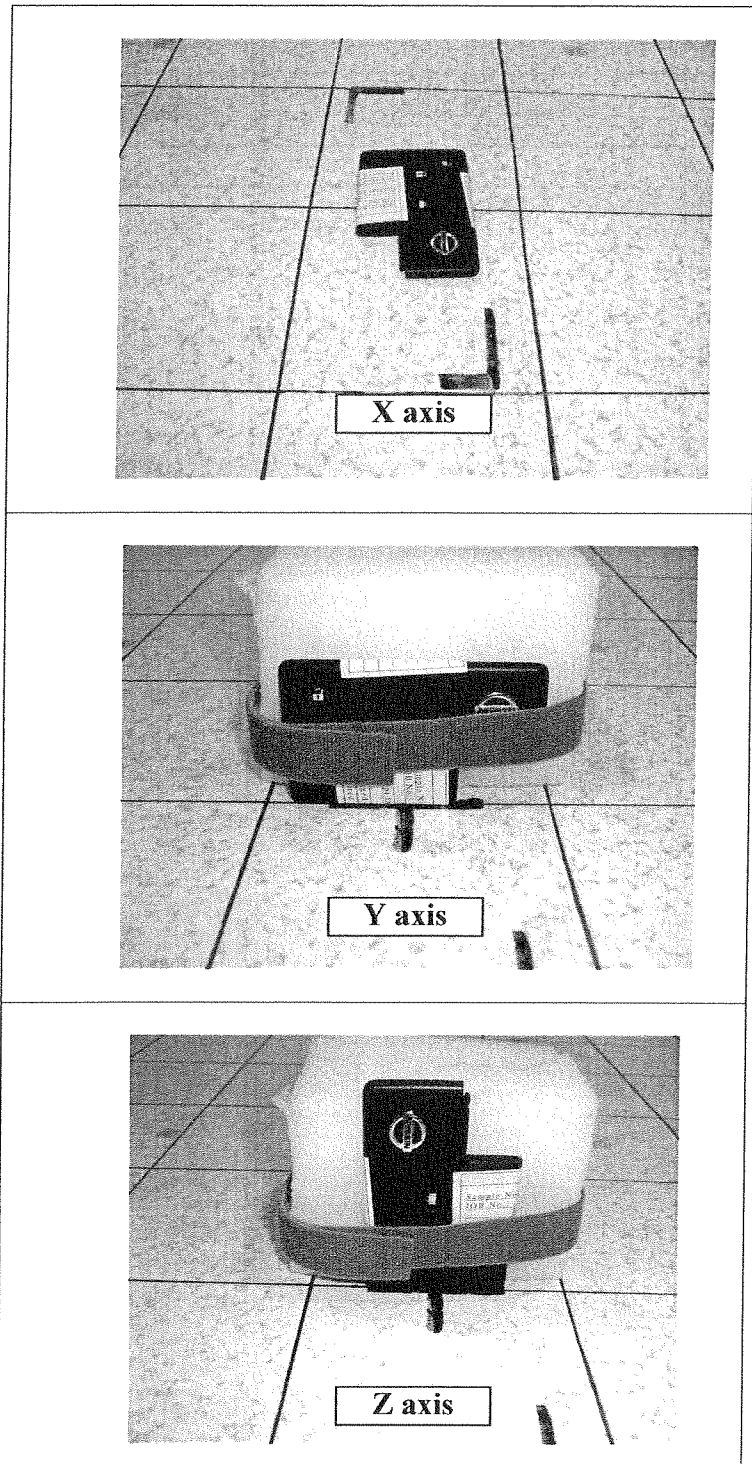
Worse case X axis (Measurement Biconical antenna Polarization :Horizontal) And Worst case Z axis (Measurement Biconical antenna Polarization: Vertical)
