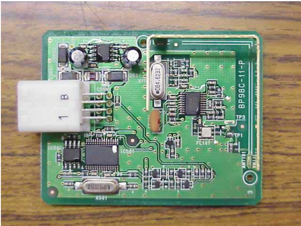
PCB Side A
