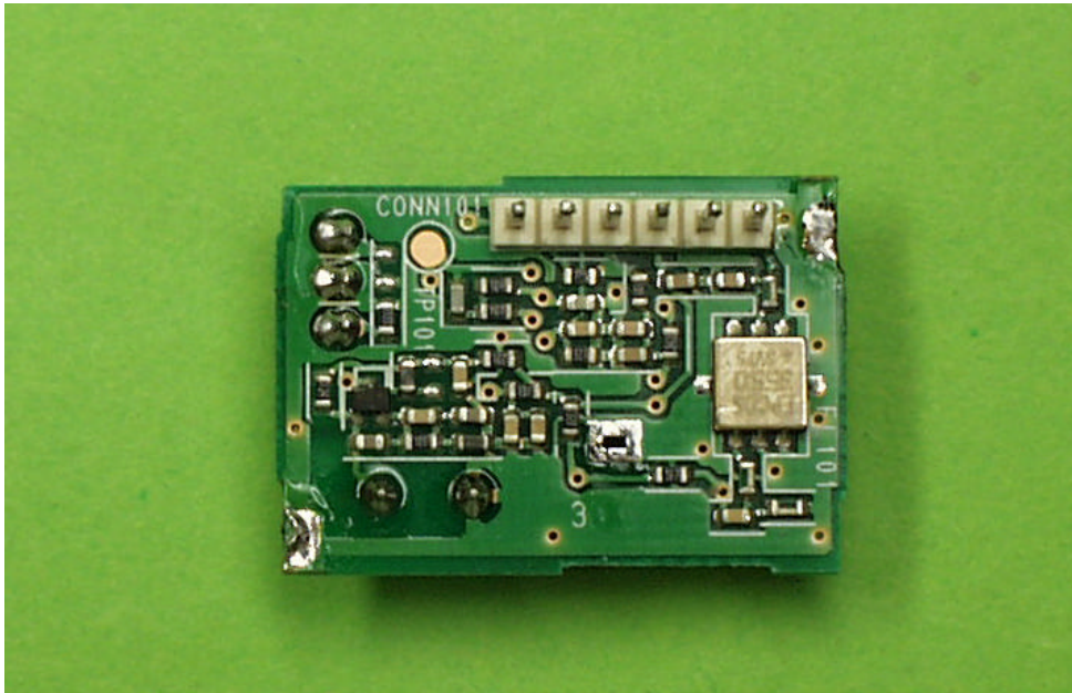
RF Module -Rear view without Shield <Tx: 125kHz>
