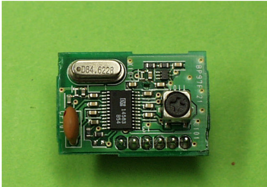
RF Module -Front view without Shield <Tx: 125kHz>
