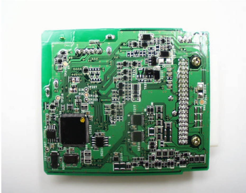
Rear view <Tx: 125kHz / Rx: 433.92MHz>
