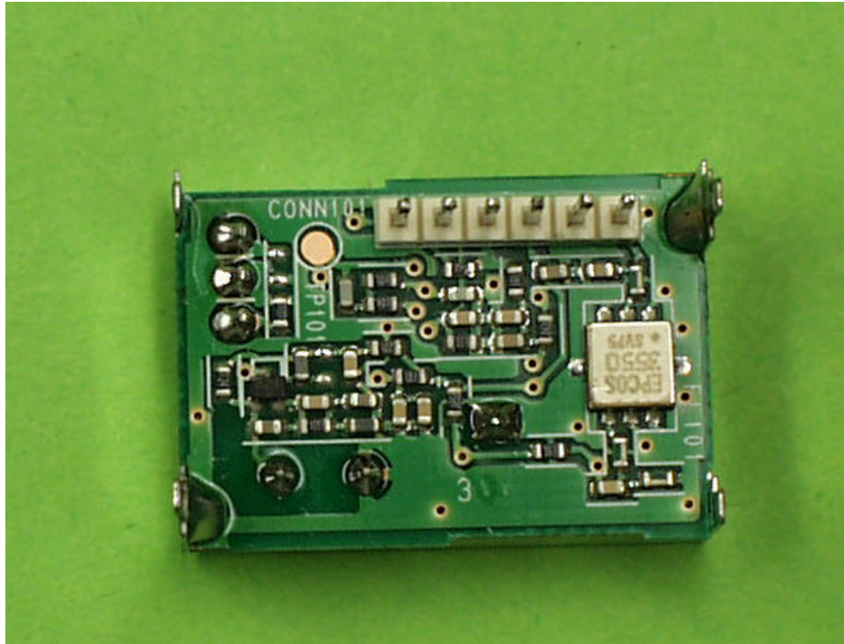
RF Module -Rear view with Shield <Tx: 125kHz>
