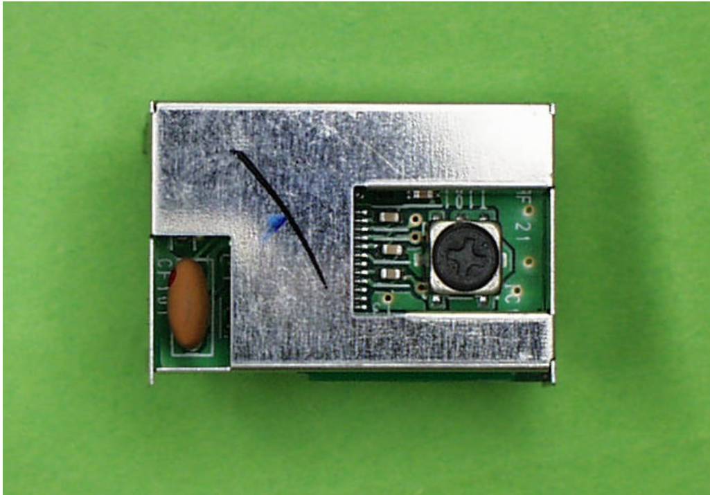
RF Module -Front view with Shield <Tx: 125kHz>
