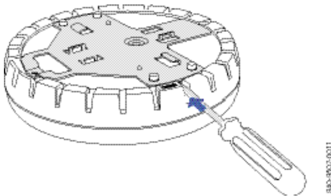
Figure 34. Step 1a—Unlocking the Bracket
