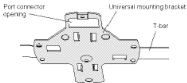
Figure 22. Step 6—Bottom View
