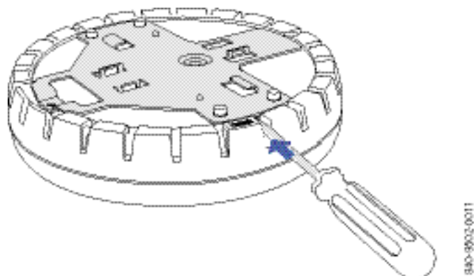
Figure 11. Step 5—Unlocking the Bracket
