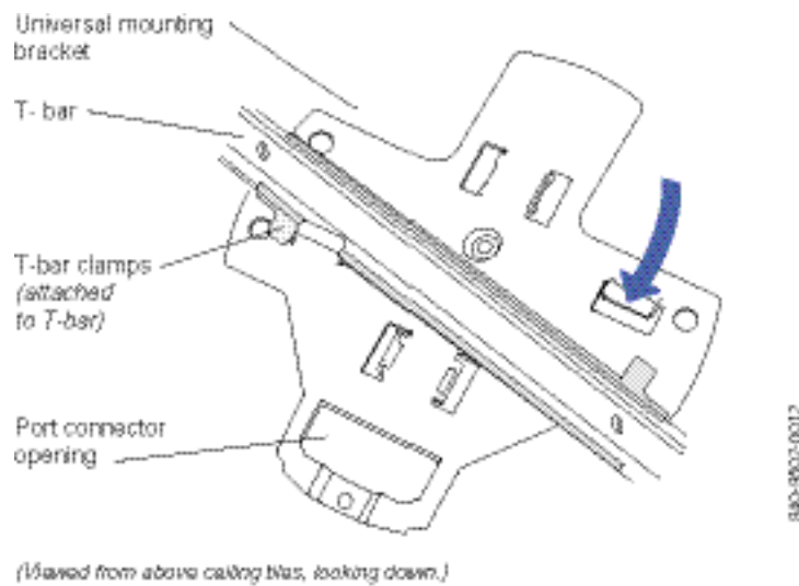
Figure 21. Step 6—Top View
