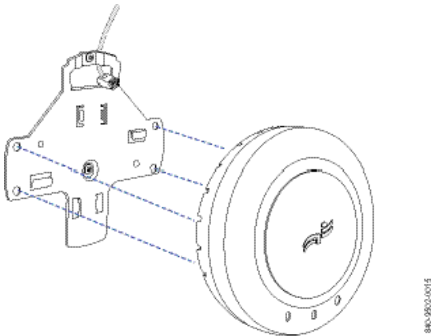
Figure 31. Steps 5 and 6—Bracket Placement on Solid Wall or Ceiling
