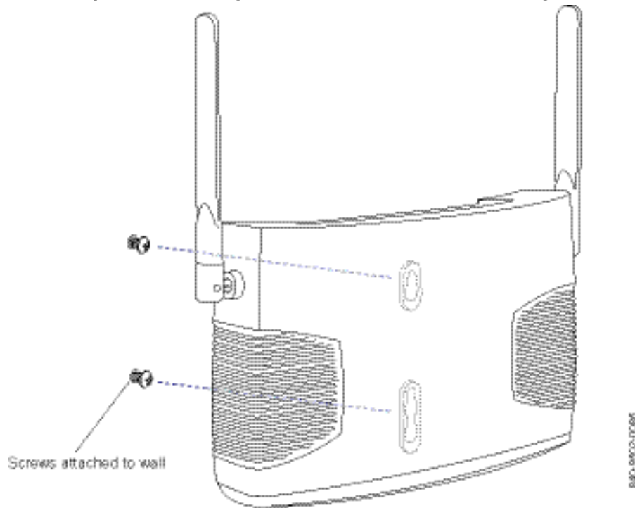
Figure 42. Step 3—Attaching the MP to the Wall or Ceiling
