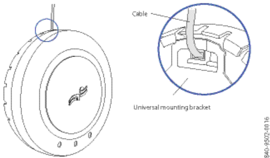
Figure 32. Step 8—Cable Placement
