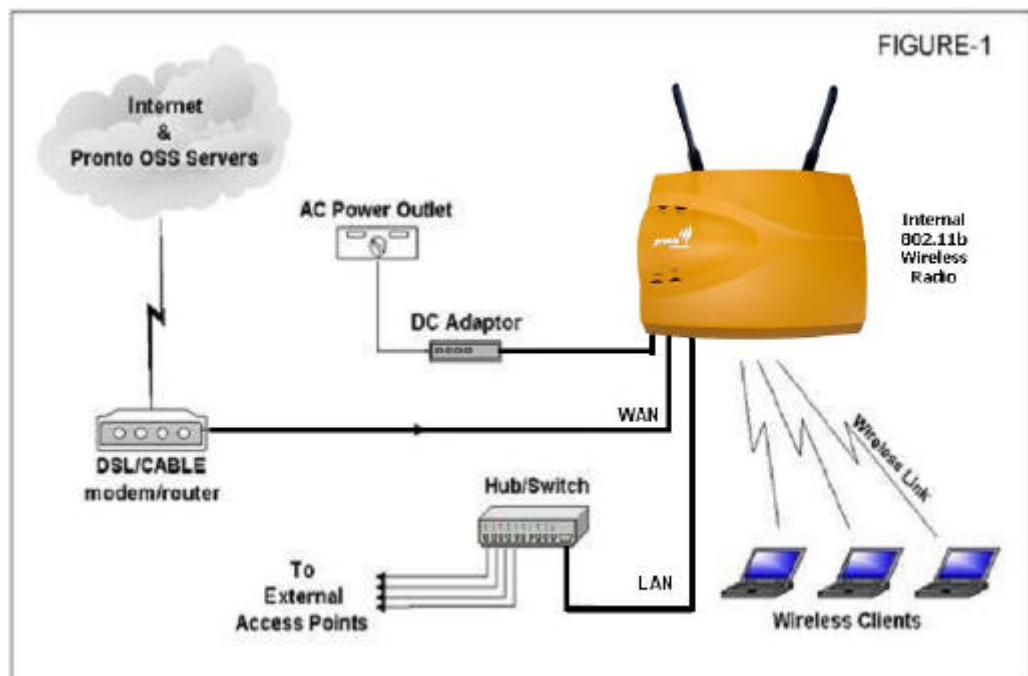
Pronto Controller Setup Diagram
