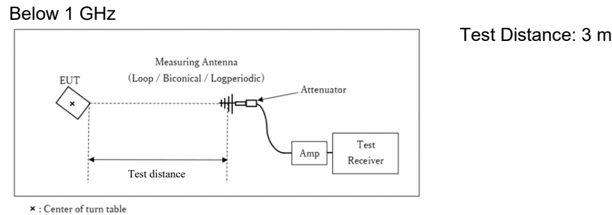
Figure 1: Test Setup
