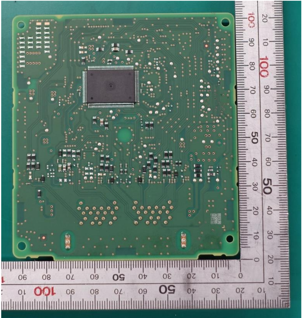
Rear
