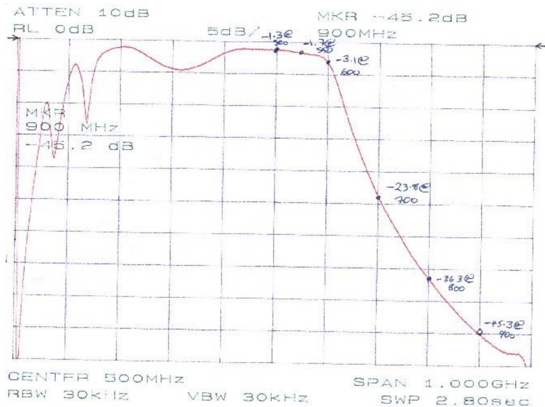
Fig (1) – LPF Response DC – 1GHz at 5dB / Division.
