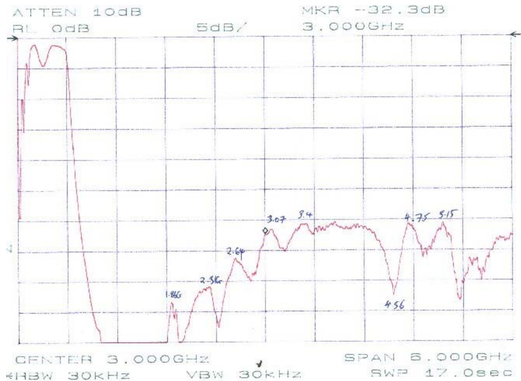
Fig (2) – LPF Response DC – 6GHz at 5dB / Division.
