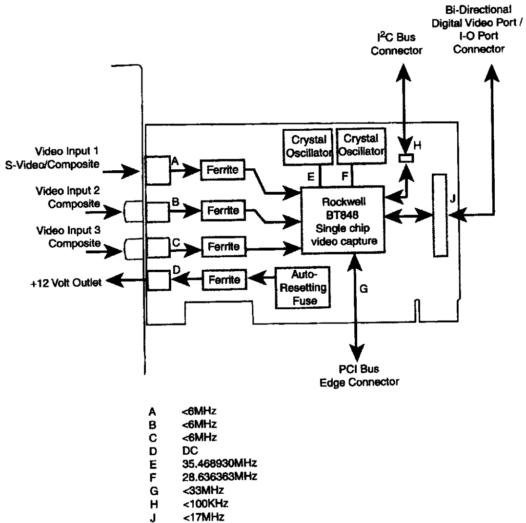
AZV30 Block Diagram
