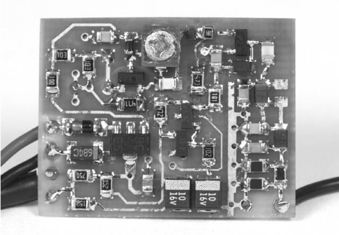
TC900 VIDEO TRANSMITTER PCB COMPONENT SIDE WITH SHIELD REMOVED
