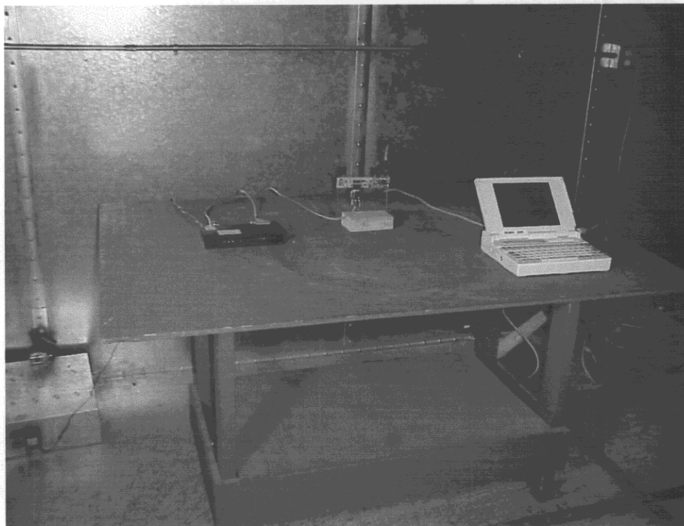
5.3 Conducted Emissions (Front View)
