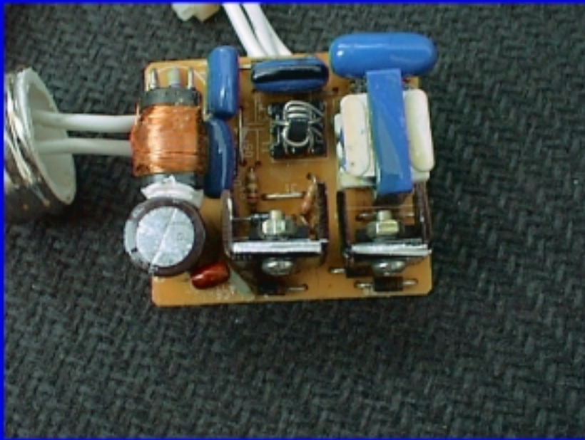
Circuit board, top
