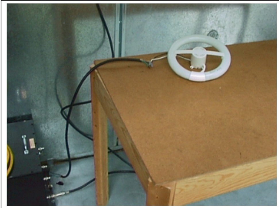
Test Setup, ECH Series
