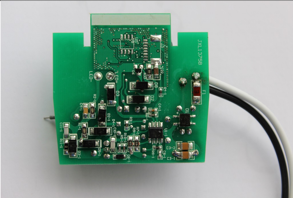
Bottom Side of the PCB.
