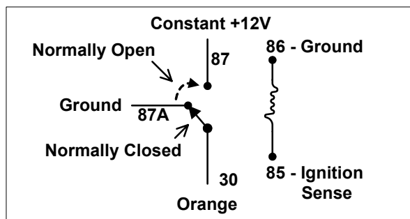
Ignition Input
