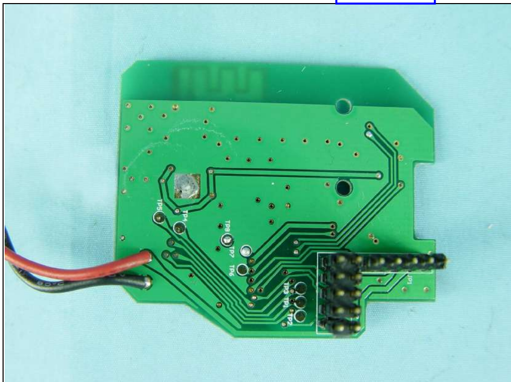
Antenna Location
