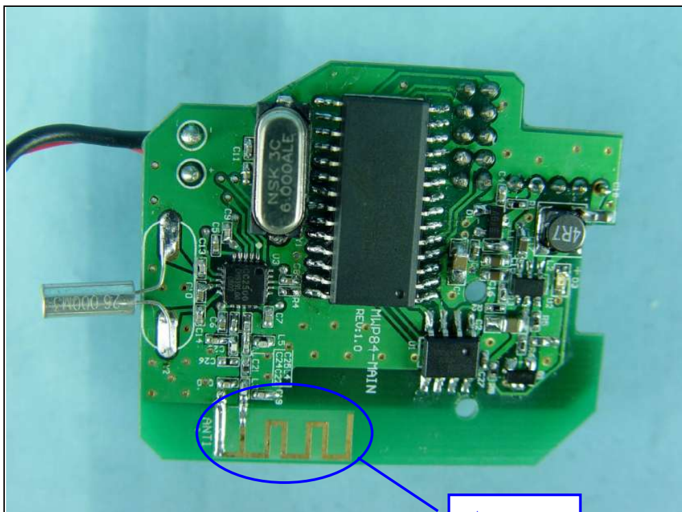
Antenna Location
