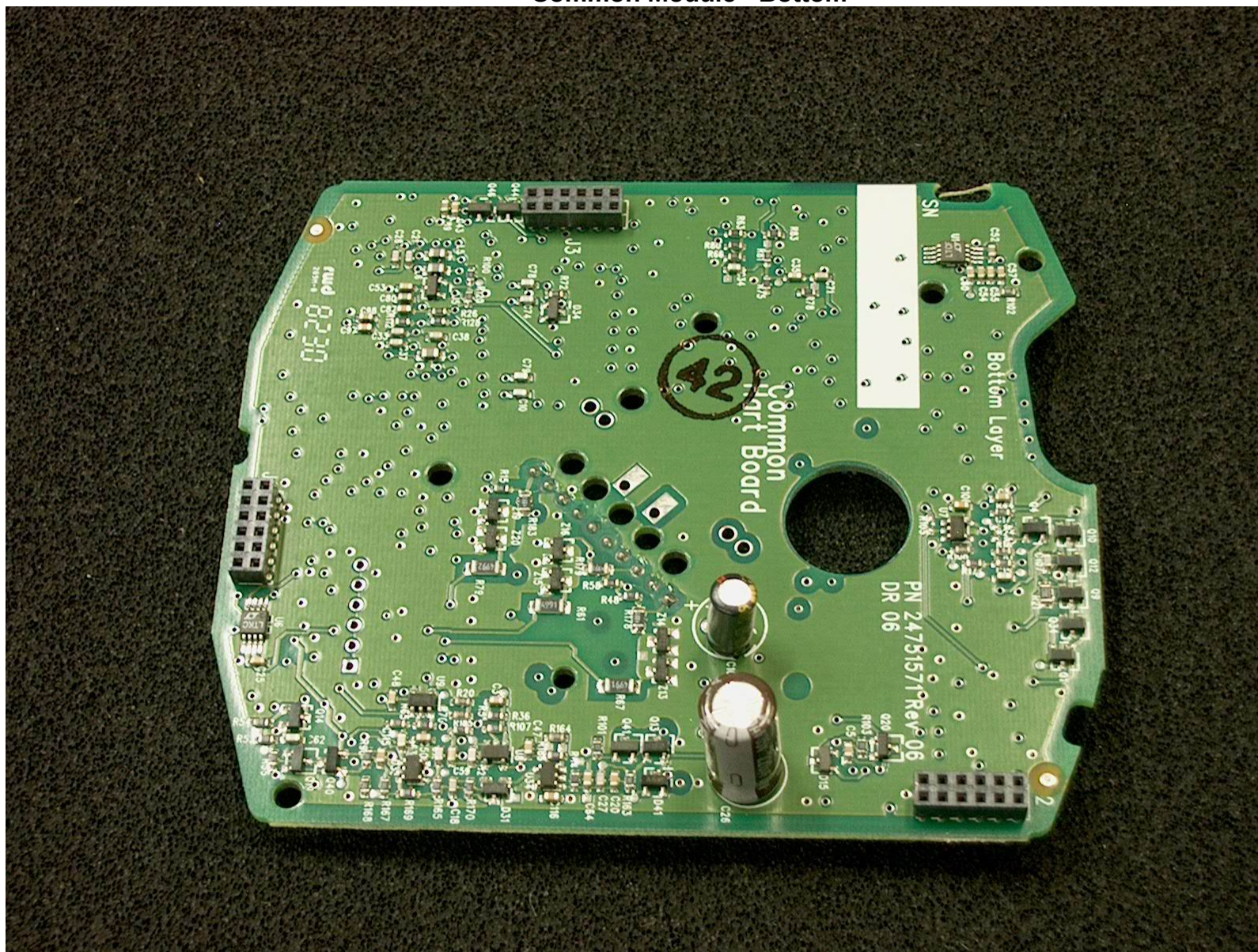
Common Module - Bottom
