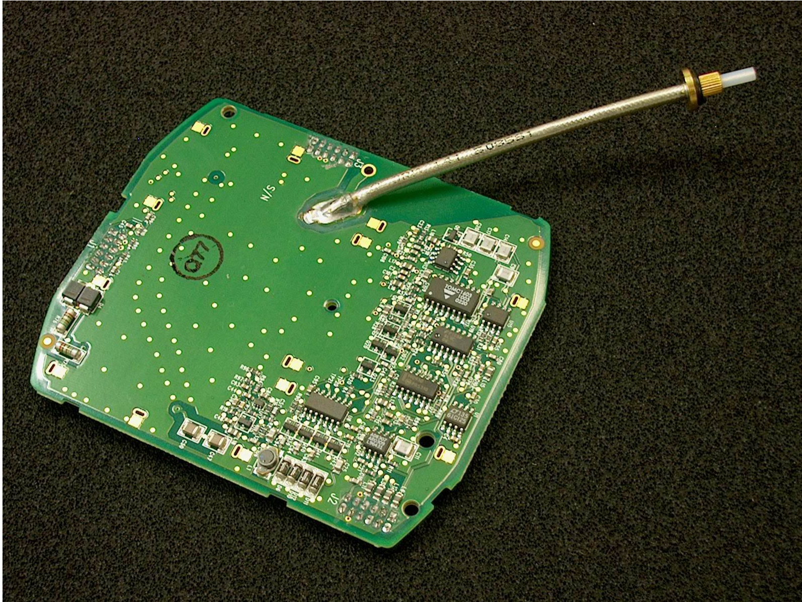
Radar Technology Module - Bottom
