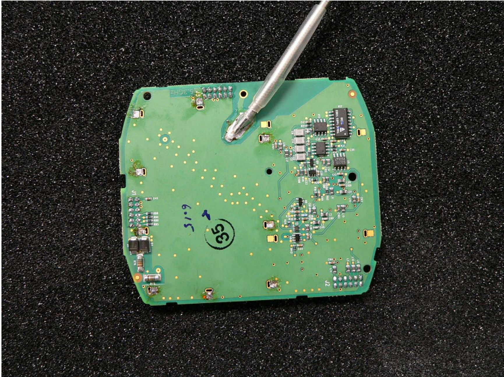
Modified Radar Board
