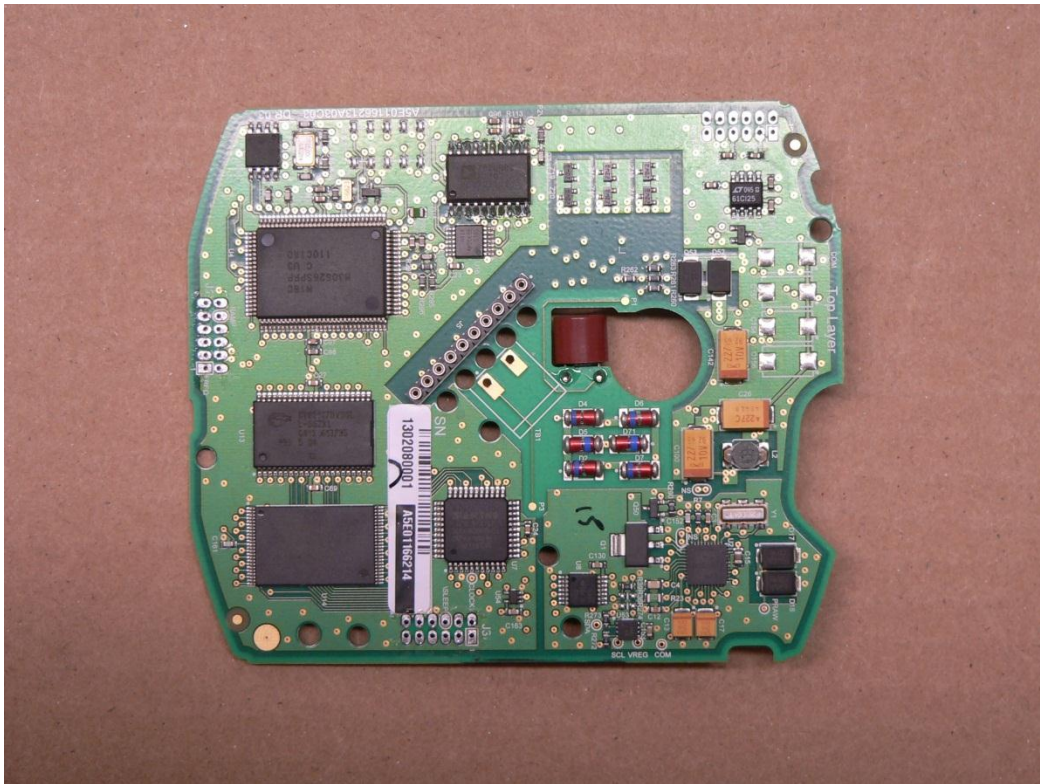
2.11 Board #5 top
