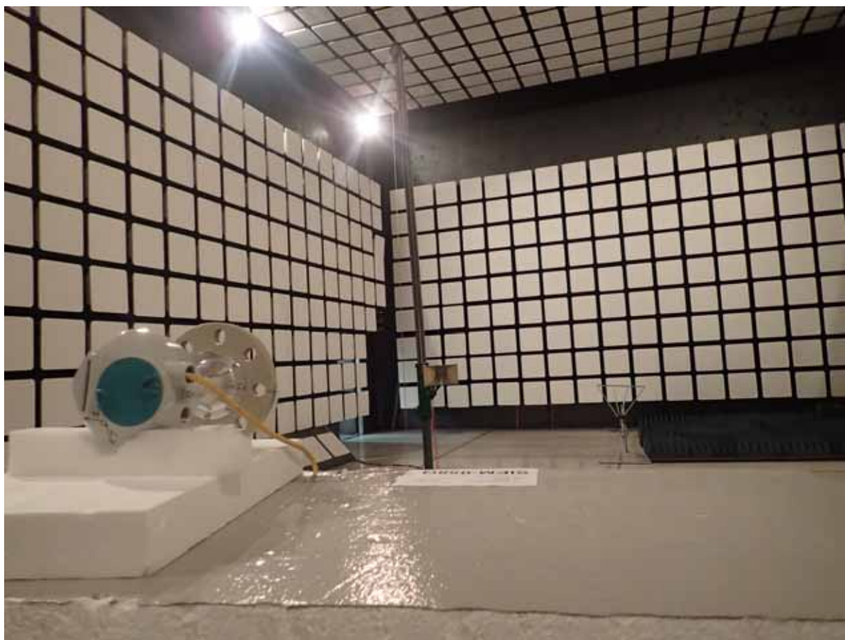
Radiated Emissions at 3 m Distance (above 1 GHz)
