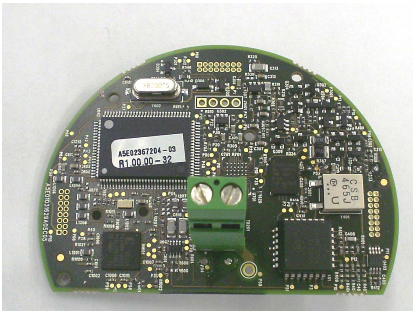
(Main Board for HART version)
